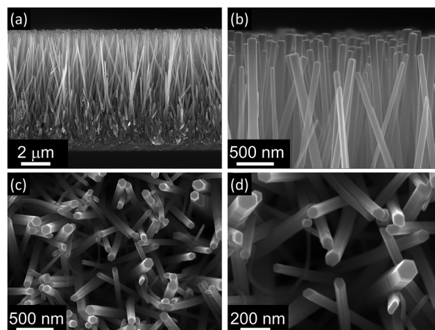
Fig. 1 Cross-section (a and b) and top-view (c and d) SEM images of ZnO nanorods grown using the hydrothermal method. After heating at 90 °C for 5 h nanorods 8.6 μm long and 79 nm wide (aspect ratio 108) with a packing density of 29 nanorod per μm 2 were obtained.
