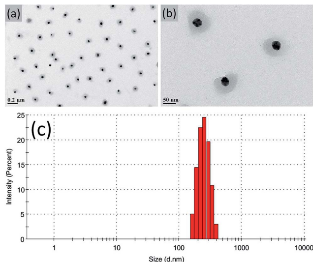
Fig. 3 TEM images (a and b) and hydrodynamic diameter distribution (c) of Ag@P(NIPAM- co -MAPTMS) hybrid microgels prepared at a NIPAM loading of 0.04 g.
