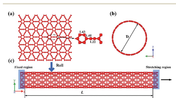
Fig. 1 A schematic diagram of: (a) a \gamma -graphyne sheet and (b) the lateral view and (c) the front view of a \gamma -GNT. The arrow indicates that uniform strain was applied along the x-axis direction.
