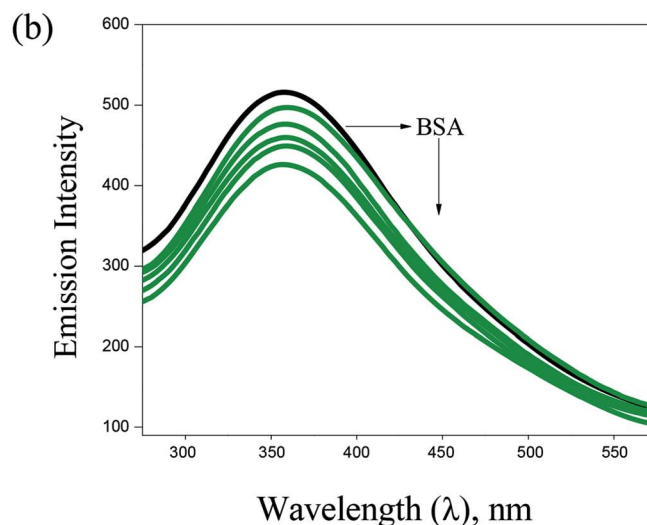
Fig. 7 Fluorescence spectra of BSA (10 \mu\text{M} , \lambda_{\text{ex}} = 280 \text{ nm} , \lambda_{\text{em}} = 570 \text{ nm} ) in the presence of increasing concentrations of 2 (a) and 3 (b). Arrow shows that the emission intensity changes upon increasing the concentration of the complexes.
