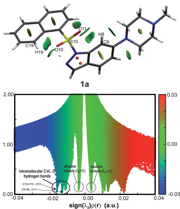
Fig. 6 Gradient isosurfaces representing intramolecular interactions (top) and corresponding plots of the reduced density gradient (RDG) vs. the electron density multiplied by the sign of the second Hessian eigenvalue (bottom) for the isolated molecule 1a (as an example). The shape of the domains is correlated with the strength of the interaction. Broad green/blue disk-shaped domains indicate weak attractive ( \lambda_2 < 0 ) and green repulsive ( \lambda_2 > 0 ) interactions (represented as blue/green and green spikes in the plot below). Delocalized electrons of aromatic groups are represented by egg-shaped domains. Gradient surfaces correspond to s = 0.1 \text{ a.u.} The color scale in the plot corresponds to -0.04 < \rho < 0.04 \text{ a.u.}
