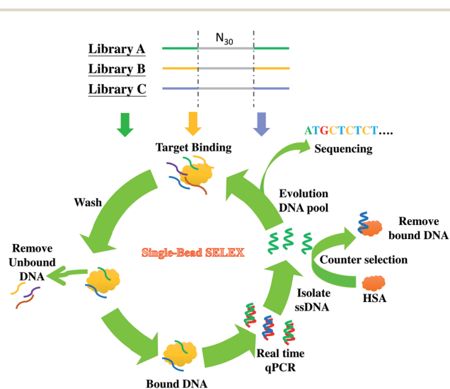
Scheme 1 Selection of anti-AMACR aptamers from three DNA libraries (N 30 ) with different primers by single-bead SELEX.
