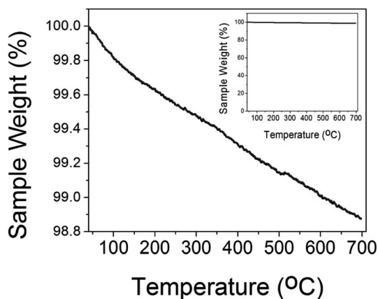
Fig. 3 TGA data of different CuO( A_{24\text{ h-C}_4\text{ h}} ) nanoparticles prepared by aging for 24 h followed by the urea-assisted homogenous precipitation at 90^\circ\text{C} for 2 h and subsequent calcination in ambient air at 400^\circ\text{C} for 4 h. The inset is the full scale TGA plot.
