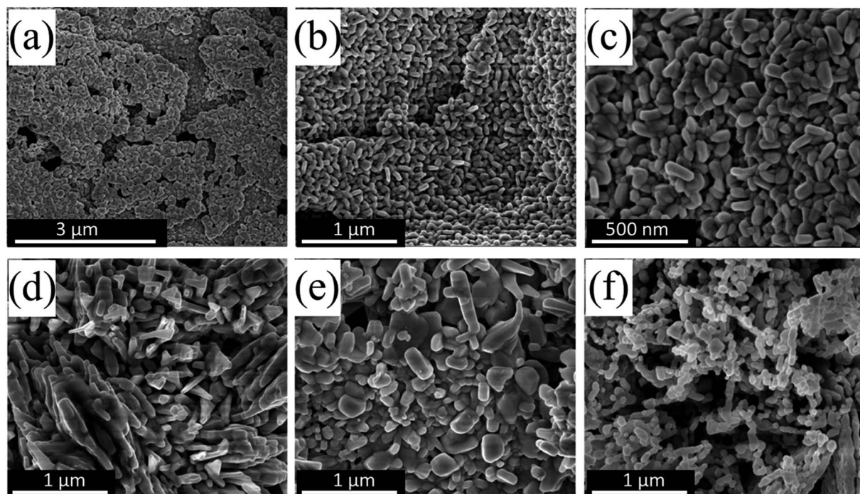
Fig. 1 SEM images of (a–c) \text{CuO}(\text{A}_{24\text{h}}-\text{C}_{2\text{h}}) , (d) \text{CuO}(\text{A}_{2\text{h}}-\text{C}_{2\text{h}}) , (e) \text{CuO}(\text{A}_{72\text{h}}-\text{C}_{2\text{h}}) and (f) \text{CuO}(\text{A}_{24\text{h}}-\text{C}_{4\text{h}}) nanoparticles prepared by aging the reaction mixture for different times followed by the urea-assisted homogenous precipitation (UAHP) at 90 °C for 2 h and subsequent calcination at 400 °C in ambient air.
