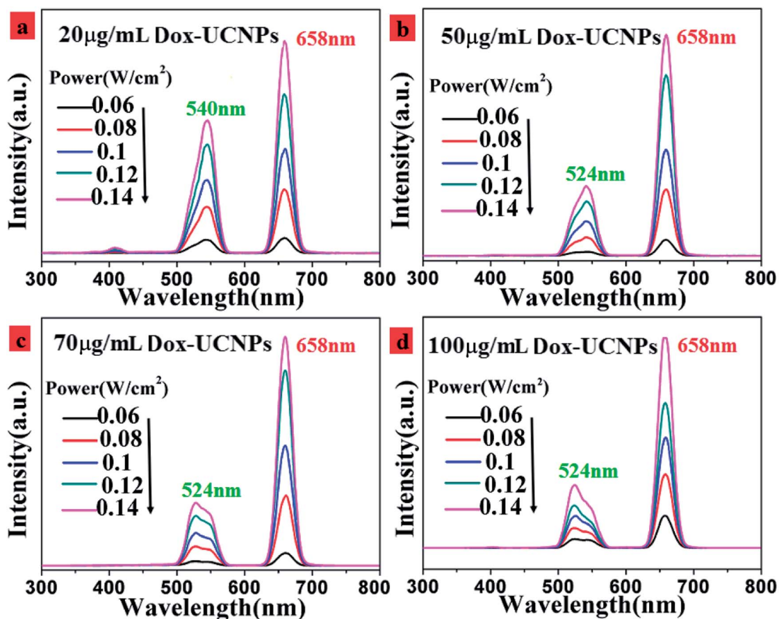
Fig. 7 UC luminescence spectra of \text{NaGdF}_4\text{:18\%Yb}^{3+}, 2\%\text{Er}^{3+} @ \text{NaYF}_4 core/shell particles in the with different concentrations of Dox. (a) 20 \mu\text{g mL}^{-1} ; (b) 50 \mu\text{g mL}^{-1} ; (c) 70 \mu\text{g mL}^{-1} ; (d) 100 \mu\text{g mL}^{-1} at 980 nm-excitation under different laser powers.
