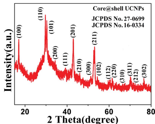
Fig. 3 XRD spectrum of \text{NaGdF}_4\text{:18% Yb}^{3+},2%\text{Er}^{3+}@NaYF_4 core/shell particles.
