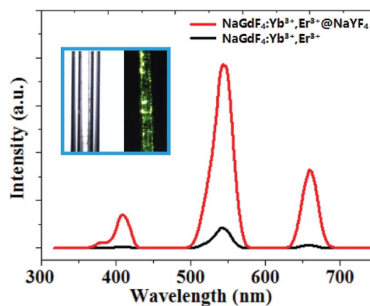
Fig. 4 Room temperature upconversion emission spectrum of core/shell \text{NaGdF}_4\text{:18% Yb}^{3+},2%\text{Er}^{3+}@NaYF_4 and bare \text{NaGdF}_4\text{:18% Yb}^{3+},2%\text{Er}^{3+} nanoparticles. The inset: the photograph of core/shell UCNPs dispersed in CGT under the 0.08\text{ W cm}^{-2} laser power at 980 nm excitation.
