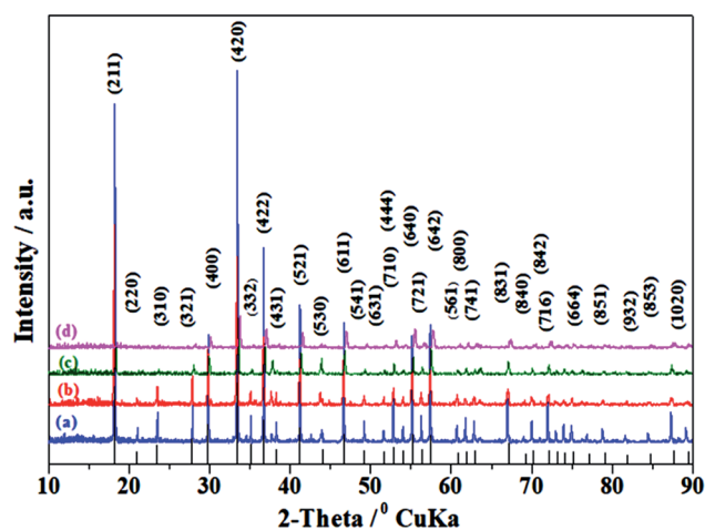
Fig. 8 XRD of \text{C}_{12}\text{A}_7-x\text{V}_x:e^- , where x = (a) 1, (b) 0.75, (c) 0.50, (d) 0.25 , heated at 1550 °C for 1 h. The lines on the x-axis correspond to the peak positions for pure \text{C}_{12}\text{A}_7 .
