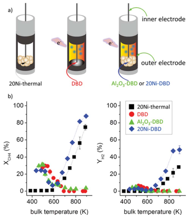
Fig. 6 (a) Reaction environments for the CH 4 reforming and (b) profiles of CH 4 conversions ( X_{\text{CH}_4} ) and H 2 yields ( Y_{\text{H}_2} ) at various reaction environments obtained via bulk temperature controls. Reproduced from ref. 200 with permission from American Chemical Society, copyright 2016.
