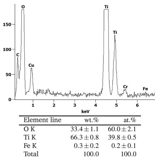
Fig. 2 The EDX-analysis of the area marked with A in Fig. 1.
