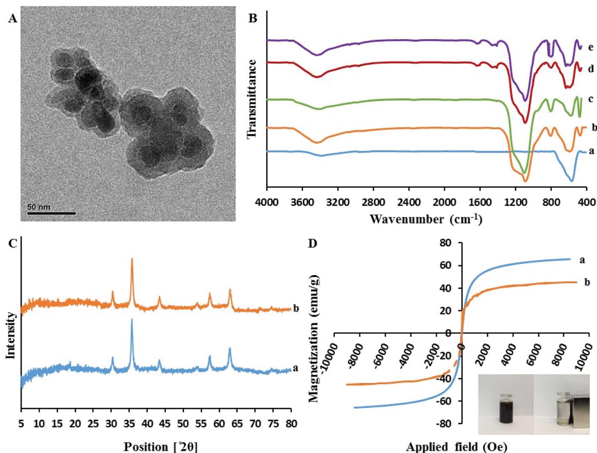
Fig. 3 (A) The transmission electron microscopy image of \text{Fe}_3\text{O}_4@ \text{SiO}_2@ \text{PIL-PF}_6 ; (B) The FT-IR spectra of \text{Fe}_3\text{O}_4 (a), \text{Fe}_3\text{O}_4@ \text{SiO}_2 (b), \text{Fe}_3\text{O}_4@ \text{SiO}_2@ \text{VTES} (c), \text{Fe}_3\text{O}_4@ \text{SiO}_2@ \text{PIL-Br} (d) \text{Fe}_3\text{O}_4@ \text{SiO}_2@ \text{PIL-PF}_6 (e); (C) XRD pattern of the \text{Fe}_3\text{O}_4 (a) and \text{Fe}_3\text{O}_4@ \text{SiO}_2@ \text{PIL-PF}_6 (b) nanoparticles; (D) Magnetic hysteresis loops of \text{Fe}_3\text{O}_4 (a) and \text{Fe}_3\text{O}_4@ \text{SiO}_2@ \text{PIL-PF}_6 (b).
