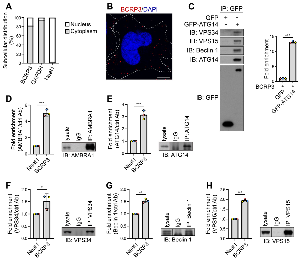
Fig. 4 BCRP3 is mainly distributed to the cytoplasm and binds VPS34 complex. A Subcellular localization of BCRP3 in HeLa cells detected by cell fractionation followed by qRT-PCR analysis. GAPDH and Neat1 were used as cytoplasmic and nuclear RNA controls, respectively. B RNA FISH analysis of BCRP3 (red) in HeLa cells. Nuclei were stained with DAPI (blue). Bar, 10 μm. C In vitro RNA protein binding assay. GFP-ATG14 transiently expressed in 293T cells was immunoprecipitated with GFP-Trap beads and the immunocomplexes were incubated with in vitro transcribed BCRP3 . The bound RNAs were extracted and analyzed by qRT-PCR, whereas the presence of VPS34 complex components in the immunocomplexes was analyzed by Western blot (left). Data are means ± SD from three independent experiments. P values are determined by unpaired t-test, *** P < 0.001. D-H RNA immunoprecipitation assay using indicated antibodies followed by qRT-PCR analysis. Data were normalized to the IgG control and expressed as means ± SD, n = 3. P values are determined by unpaired t-test, * P < 0.05, ** P < 0.01, *** P < 0.001
