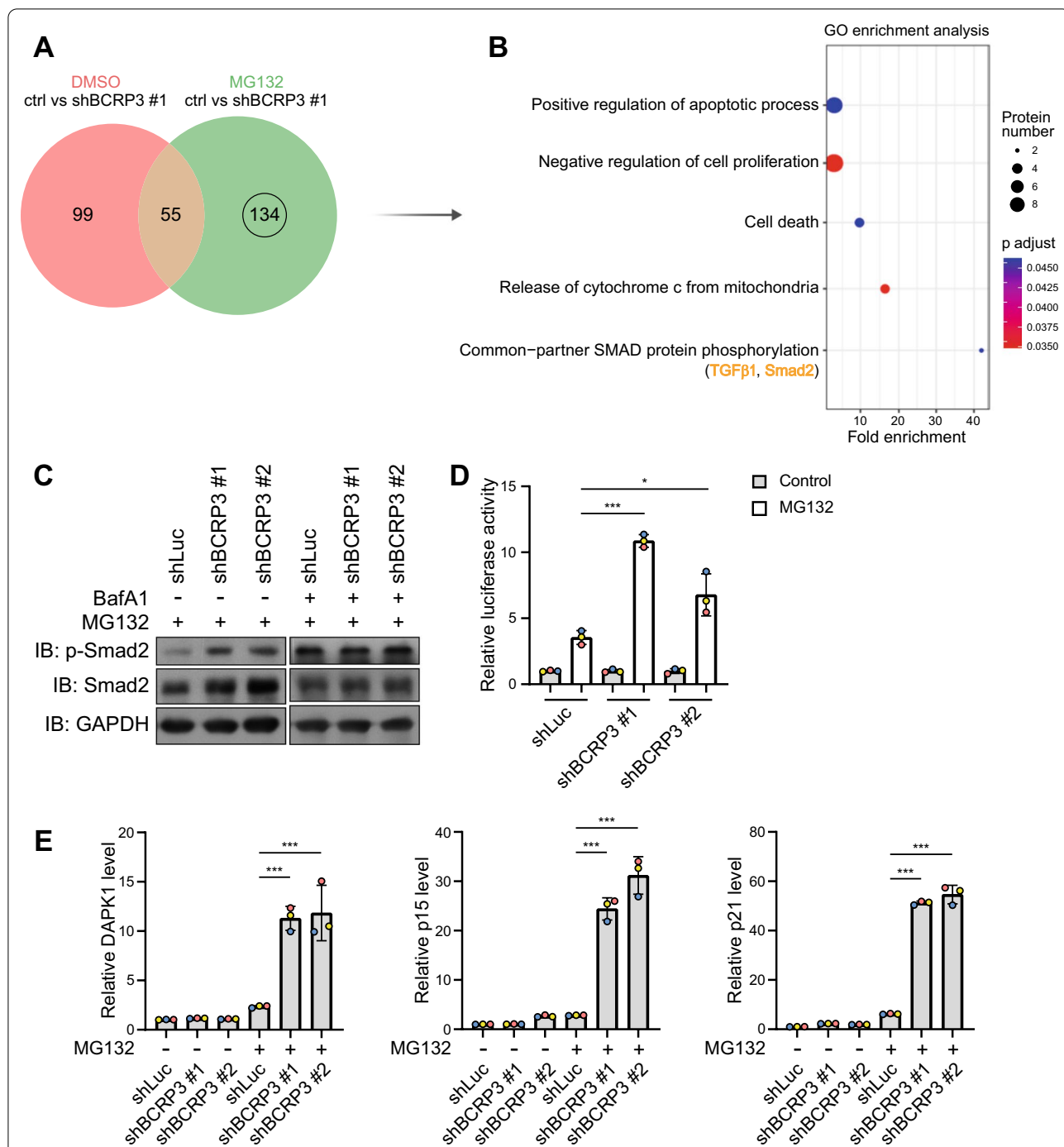
Fig. 7 BCRP3 deficiency in proteotoxicity leads to the accumulation of proteins involving in growth inhibition, cell death, and TGF- \beta /Smad2 signaling. A Venn diagram showing the numbers of enriched proteins after BCRP3 knockdown together with or without 10 \mu M MG132 treatment for 12 h. B GO enrichment analysis of the 134 proteins shown in (A) . Selective enriched GO terms are shown by the order of fold enrichment (bottom to top). C Western blot analysis of indicated proteins in control or BCRP3 -deficient HeLa cells treated with 10 \mu M MG132 together for 12 h together with or without 200 nM bafilomycin A1 for 2 h. D Control or BCRP3 -deficient HeLa cells were transfected with 4 \times SBE-Luc reporter construct, treated with 10 \mu M MG132 for 12 h and analyzed for luciferase activity. E qRT-PCR analysis of relative DAPK1 , p15 , and p21 levels in control or BCRP3 -deficient HeLa cells treated with 10 \mu M MG132 for 12 h. Data in (D) , (E) are means \pm SD from three independent experiments. P values are determined by one-way ANOVA with Tukey's post hoc test, * P < 0.05, *** P < 0.001
