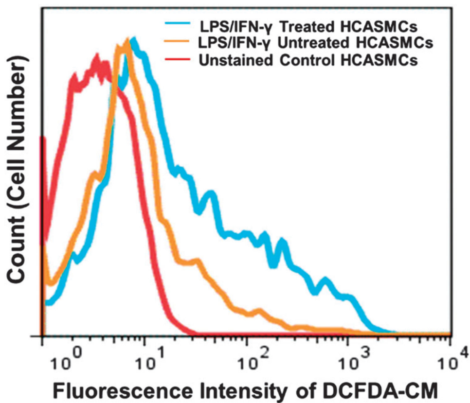
Fig. 6. Flow cytometric analysis of intracellular ROS levels in HCASMCs stained with CM- H_2DCFDA ( 10 \mu M ) after treatment with or without LPS ( 1 \mu g mL^{-1} )/IFN- \gamma (100 units per mL) for 8 h. The LPS/IFN- \gamma -treated HCASMCs showed more ROS production compared to untreated cells ( n = 3 ).
