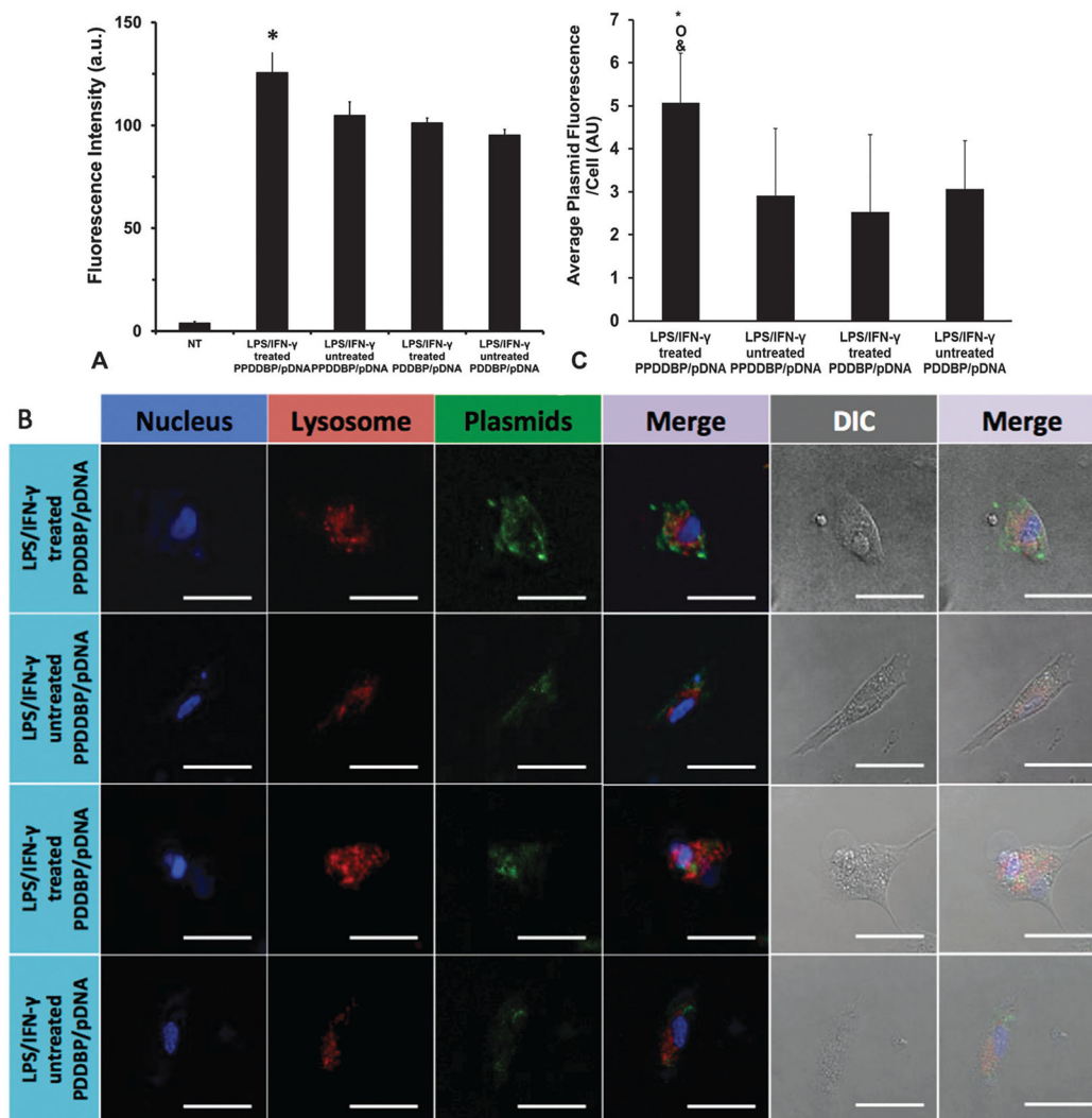
Fig. 7. Cellular uptake of polyplexes prepared using either PPDDBP or non-cleavable PDDBP with fluorescein-labeled pDNA was assessed in HCASMCs after 6 h incubation in the presence or the absence of LPS/IFN- \gamma . (A) Flow cytometry analysis indicates enhanced internalization of LPS/IFN- \gamma treated PPDDBP/pDNA polyplexes compared to other treatment groups. NT represents the non-treated group. *p < 0.05 , where * is in comparison to the other test groups. (B) Confocal images of internalized polyplexes demonstrated distribution of plasmid (green), endosomes (red), and nuclei (blue). The cells were stained with DAPI and endosomal dye LysoTracker to visualize the nucleus and endosomes, respectively. Scale bar: 50 \mu\text{m} . (C) Confocal image analysis of polyplexes supports that LPS/IFN- \gamma treated PPDDBP/pDNA condition enhance uptake of plasmids significantly compared to all three other conditions. * , o , & indicates p < 0.05 , where * is in comparison to LPS/IFN- \gamma untreated PPDDBP/pDNA, o to LPS/IFN- \gamma treated PDDBP/pDNA, and & to LPS/IFN- \gamma treated PPDDBP/pDNA, with N = 10\text{--}15 cells in each condition.
