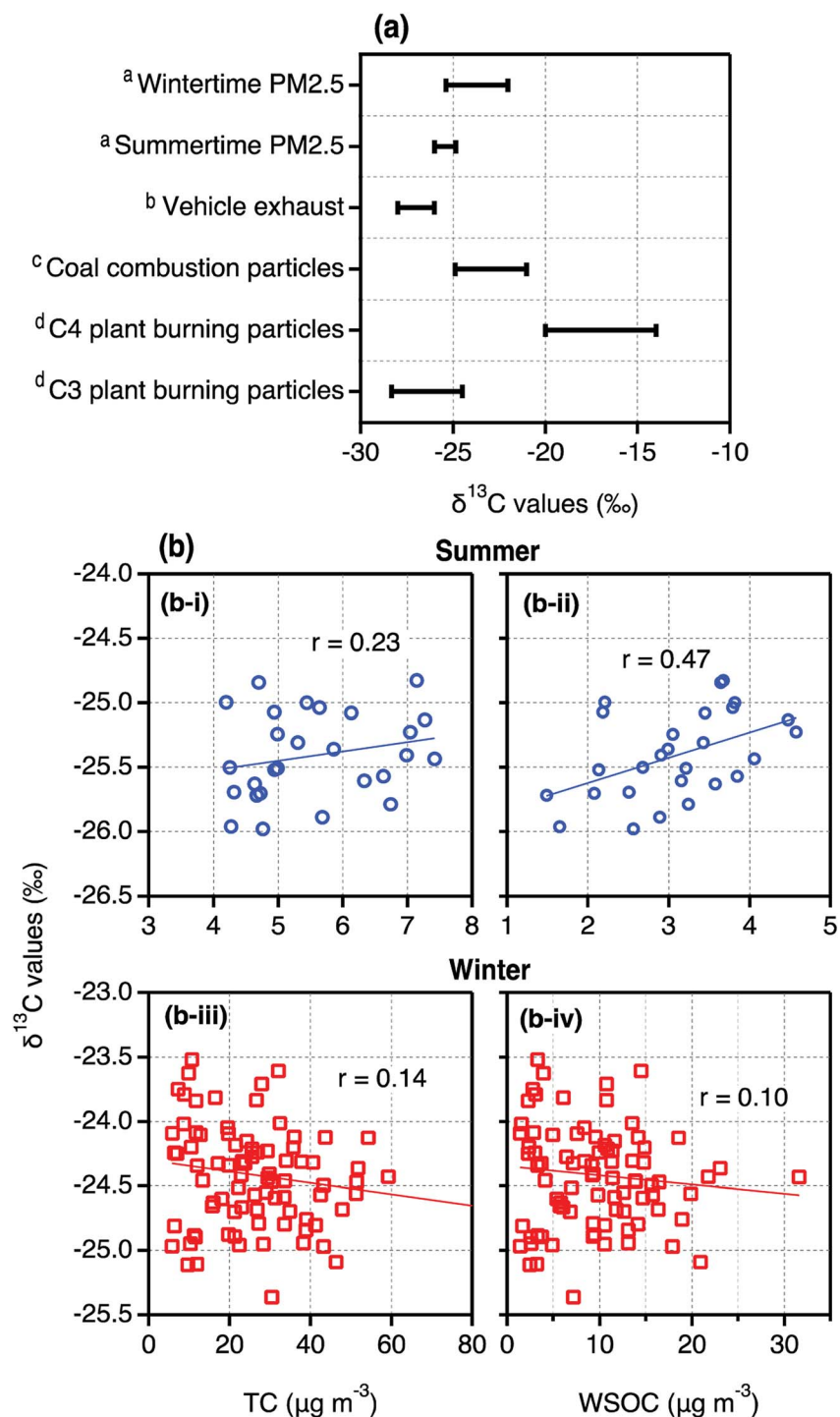
Fig. 4 (a) Ranges of \delta^{13}\text{C}_{\text{TC}} in PM 2.5 collected on day- and night-time bases in summer and winter in Tianjin, North China ( a This study) together with those in the particles emitted from specific origins ( b Widory et al. , (2004) 40 ; c Gleason and Kyser, (1984) 39 ; d Martinelli et al. , (2002) 36 ). (b) Scatter plots between \delta^{13}\text{C}_{\text{TC}} and TC and WSOC in summer and winter.
