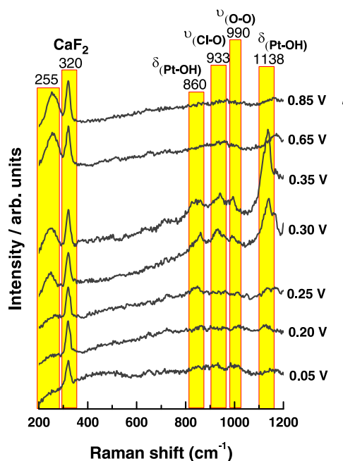
Fig. 4 Raman spectra of the hydroxyl phase at low potentials on Pt(311). Potential dependent in situ SHINERS spectra of Pt(311) electrode in 0.1 M HClO_4 electrolyte purged with Ar. The different Raman bands are highlighted by the yellow squares.
