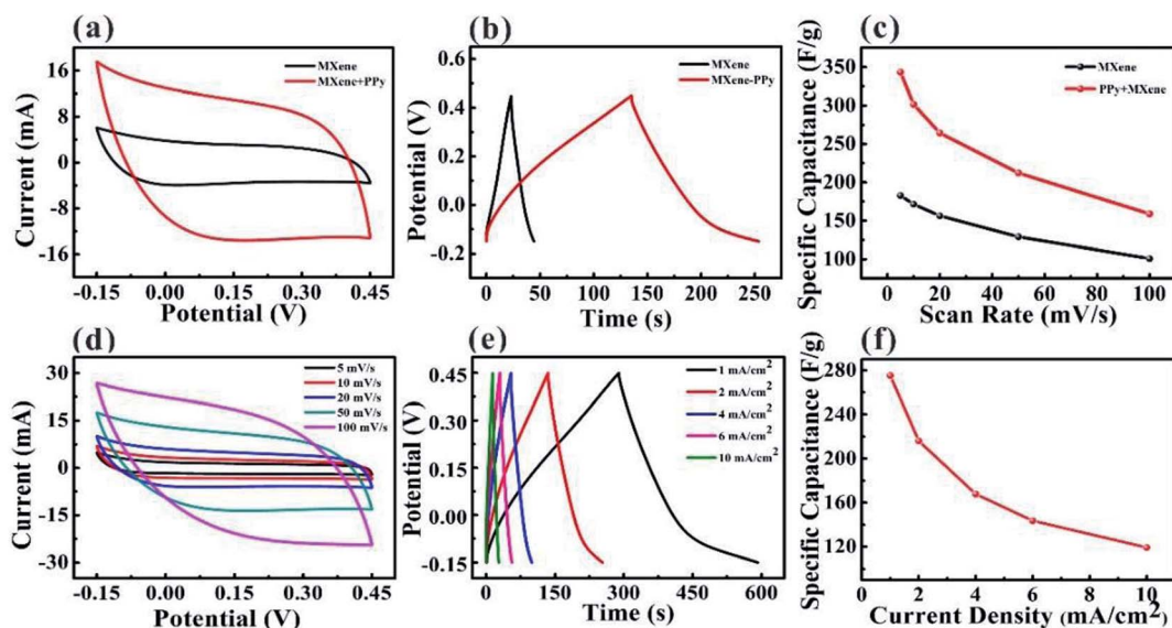
Fig. 4 Electrochemical performance of PPy-MXene coated the textile electrode. (a) The comparison of CV curves between MXene-based and PPy-MXene coated textile electrode at a scan rate of 50 \text{ mV s}^{-1} . (b) The comparison of GCD curves between MXene-based and PPy-MXene coated textile electrode under a current density of 2 \text{ mA cm}^{-2} . (c) The comparison of specific capacitance between MXene-based and PPy-MXene coated textile electrode. (d) CV curves of PPy-MXene coated textile electrode at the different scan rate. (e) GCD curves of PPy-MXene coated textile electrode at various current densities. (f) The specific capacitance of PPy-MXene coated textile electrode with respect to scan rate.
