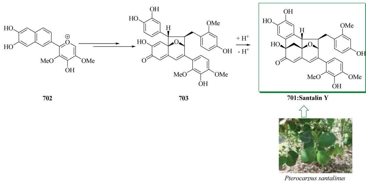
Scheme 151 Total synthesis of santalin Y 701.
