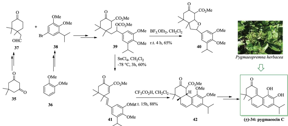
Scheme 7 Total synthesis of pygmaecocin C 34.
