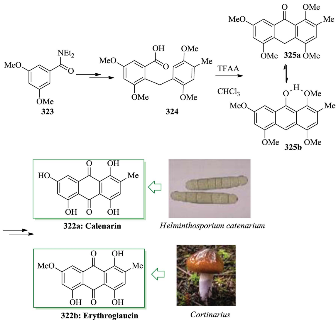
Scheme 65 Total synthesis of catenarin 322a and erythroglauцин 322b.
