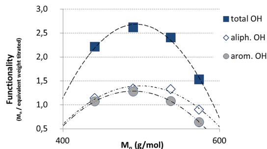
Fig. 8 Estimated functionalities of the precipitated lignin fractions.
