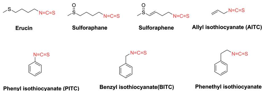
Fig. 1 The representatives of naturally occurring isothiocyanates.
