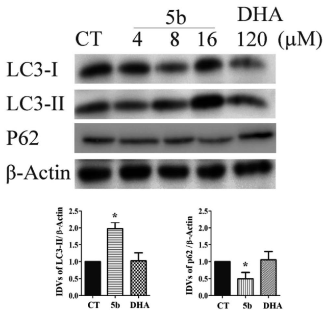
Fig. 7 5b induces autophagy in human GBM cells. Cells were treated with the indicated concentrations of 5b and DHA for 16 h. The proteins were collected for western blot assay with LC3B, p62 and \beta -actin antibodies. The result was obtained by three different independent experiments.
