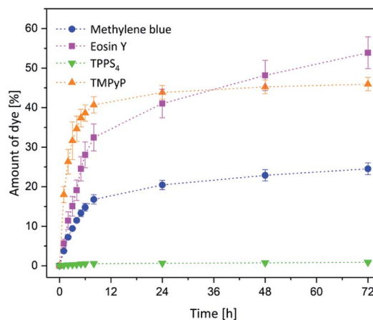
Fig. 8 Release of methylene blue (blue dot), eosin y (pink square), TMPyP (orange bottom-up triangle) and TPPS 4 (green triangle).
