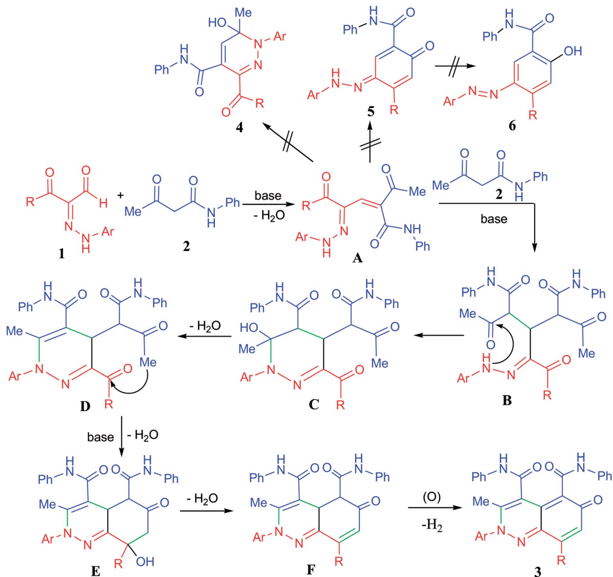
Scheme 3 Proposed mechanism for the annulation pathway.
