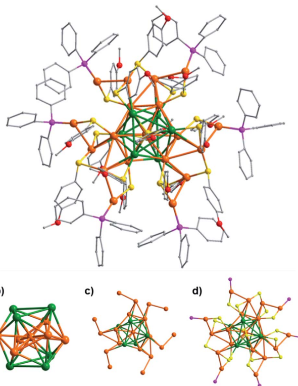
Fig. 2 (a) Molecular structure of \text{Au}_{19}\text{Ag}_6 . Au orange, Ag green, P purple, S yellow, C gray, and O red. (b) The centered icosahedral \text{Au}_7\text{Ag}_6 core. (c) \text{Au}_7\text{Ag}_6 with the 12 exterior Au atoms. (d) \text{Au}_7\text{Ag}_6 with three V-shaped [\text{Au}_2(\text{SR})_3] staples and six [\text{P}-\text{Au}-\text{SR}] staples.
