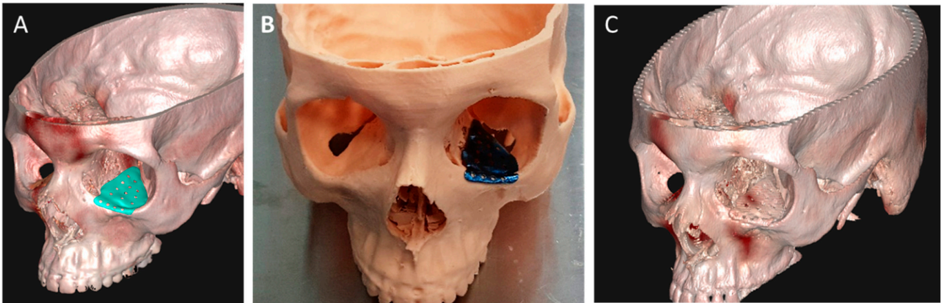
Figure 6. PSI design and 3D printing used for orbital floor reconstruction. VSP-based mirroring is utilized to design PSI for orbital floor reconstruction (A). Designed titanium implant fabricated via SLS 3D printing (B). Post-operative 3D imaging depicts accuracy of implant adaptation to the damaged anatomy (C).
