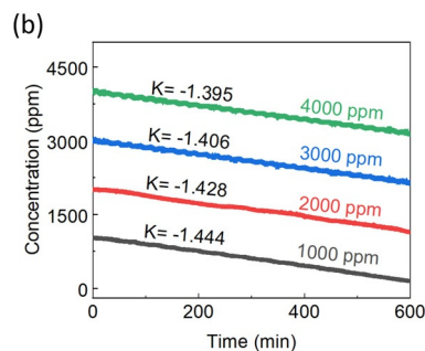
Figure 5 ... (b) corresponding salt concentration variation in the diluted stream at 0.25 \text{ mA cm}^{-2} current density.
