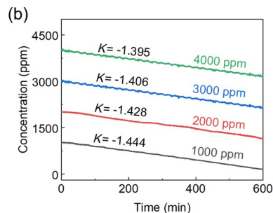
Figure 5 ... (b) corresponding salt concentration variation in the diluted stream at 0.25 \text{ mA cm}^{-2} current density.
