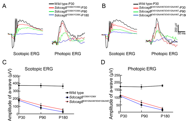
Figure 4 Scotopic and photopic electroretinograms (ERG) of rod-cone photoreceptor degeneration in Sdccag8 Y236X/Y236X and Sdccag8 E451GfsX467/E451GfsX467 mice A, B: Representative traces of scotopic (left) and photopic (right) ERG responses under 1.30 log cd-s/m 2 light stimuli recorded from wild-type mice at P30, as well as Sdccag8 Y236X/Y236X (A) and Sdccag8 E451GfsX467/E451GfsX467 (B) mice at P30, P90, and P180, indicating progressive visual dysfunction of rods and cones in knock-in mice. C, D: Average a-wave amplitudes of scotopic ERG responses (C), and average b-wave amplitudes of photopic ERG responses (D) under 1.30 log cd-s/m 2 light stimuli recorded from wild-type and knock-in mice at P30, P90, and P180, revealing rapid progressive visual dysfunction of photoreceptors with earlier onset in rods. n=3-7 .
