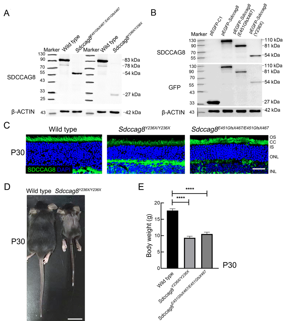
Figure 2 Sdccag8 knock-in mice carrying a hypomorphic allele with growth retardation
