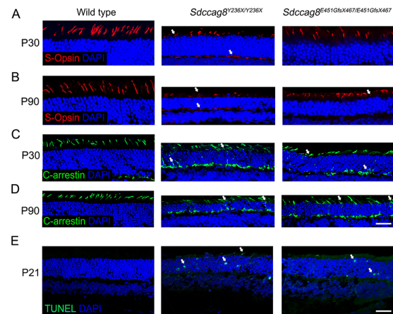
Figure 6 Immunolocalization of cone phototransduction-related proteins in Sdccag8 Y236X/Y236X and Sdccag8 E451GfsX467/E451GfsX467 mouse retinas
