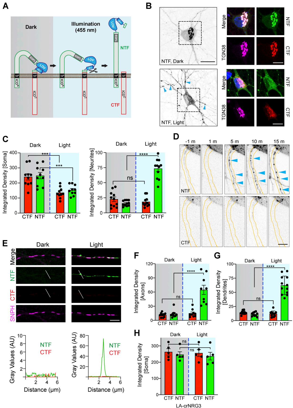
Figure 2. Light-dependent processing of LA 143 -NRG3 and its trafficking to somato-dendritic compartments and axons. (A) Illustration of light-induced conformational changes in LA 143 -NRG3 that enable BACE1 processing of proNRG3. (B) Representative post-fixation images of neurons transfected with LA 143 .
