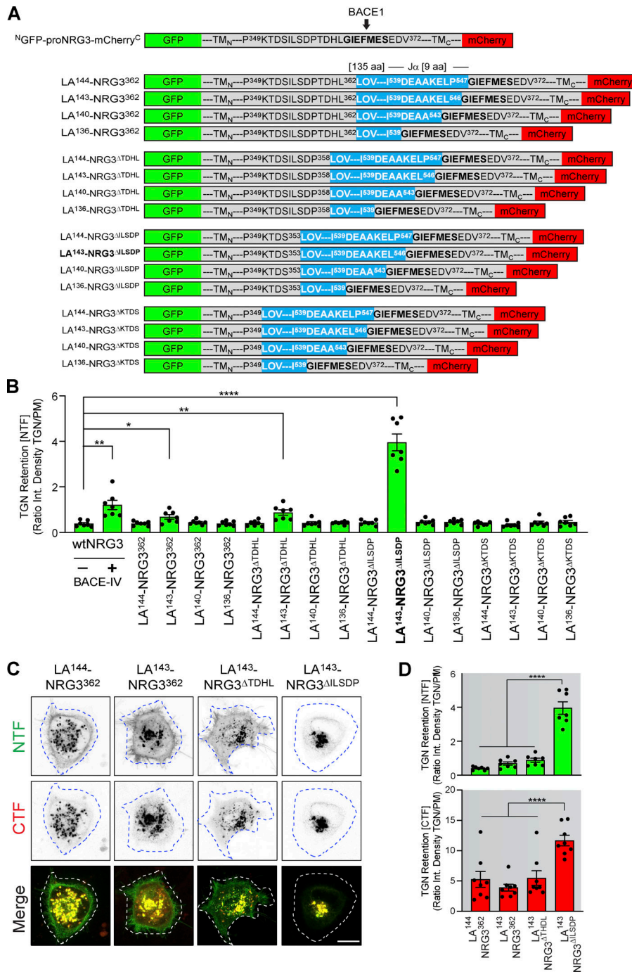
Figure S3. Generation and validation of a photoactivatable proNRG3 cleavage reporter (LA-NRG3). (A) Schematic overview of proNRG3-LOV2/J α fusion proteins tested to derive a configuration with photoactivatable BACE1 processing properties. Fusion constructs varied with regards to the LOV2/J α insertion site and number of deleted residues in proNRG3 (carboxyl-terminal to L 362 [no deletion], P 358 [ΔTDHL], S 353 [ΔILSDP], or P 349 [ΔKTDS]), as well as the extent of carboxyl-terminal deletions of the LOV2 J α helix, ranging from 0 in LA 144 to 8 in LA 136 (superscript numbers indicate the overall length of the LOV2/J α moiety). All fusion proteins are based on N GFP-proNRG3-mCherry C (shown above; BACE1 site indicated). LOV2/J α -encoding residues are shown in blue. Superscript numbers denote amino acid positions relative to their native proteins (proNRG3 and A. sativa phototropin 1, respectively). (B) Effect of LOV2/J α insertion on NRG3 accumulation at the PM in transfected HEK293 cells. GFP fluorescence intensities at TGN and PM were measured under dark conditions and used to derive TGN over PM ratios illustrating the extent of retention in the TGN. The LA 143 -NRG3 ΔILSDP variant (bold) showed the highest ratio indicative of maximum retention. As controls, TGN retention of proNRG3 lacking the LOV2/J α domain after 24 h of BACE1 inhibition by BACE-IV (1 μM) is included. Data are plotted as signal intensity ratios and represent the mean ± SEM from three independent experiments (n = 7 cells). (C) Representative images showing subcellular NRG3 NTF/CTF distribution in HEK293 cells transfected with LA 144 -NRG3 362 , LA 143 -NRG3 362 , LA 143 -NRG3 ΔTDHL , and LA 143 -NRG3 ΔILSDP under dark conditions. Note the very low NTF signal for LA 143 -NRG3 ΔILSDP in the PM. (D) Quantitative analysis of experiment shown in C. TGN retention values are plotted as ratios of integrated green or red fluorescence pixel intensities in the TGN over the PM and support the notion that LA 143 -NRG3 ΔILSDP accumulates in the TGN as an unprocessed protein. Data represent the mean ± SEM from three independent experiments (n = 8 cells). Scale bar: 10 μm. *, P < 0.05; **, P < 0.01; ****, P < 0.0001 (one-way ANOVA).
