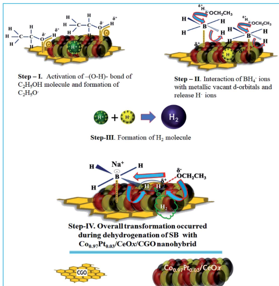
Fig. 10 The proposed catalytic mechanism for the dehydrogenation of SB with the \text{Co}_{0.97}\text{Pt}_{0.03}/\text{CeO}_x/\text{CGO} nano hybrid.
