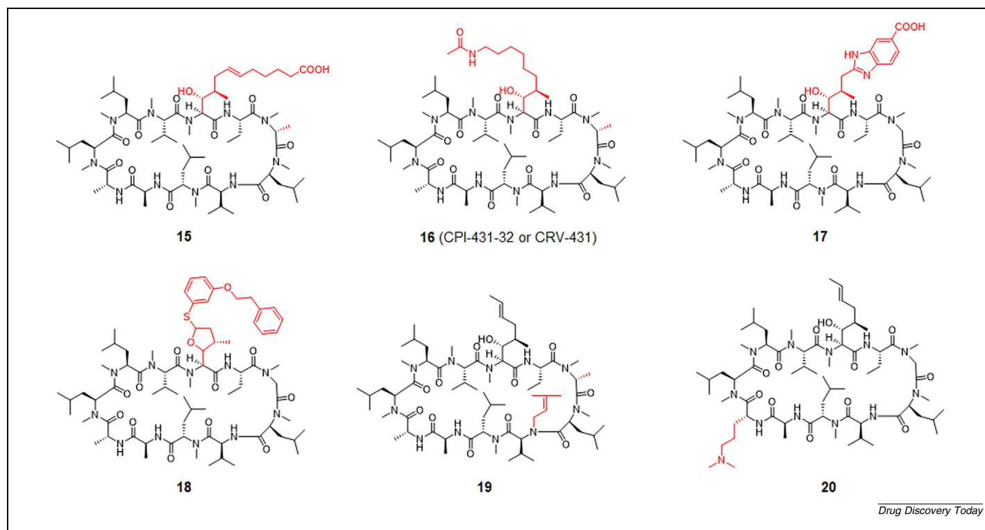
FIGURE 5 Chemical structure of CsA derivatives, including compounds 15 to 20 . In compounds 15 and 16 P1 and P3 are modified; in compounds 17 and 18 P1 is modified; in compound 19 P3 and P5 are modified; and in compound 20 P8 is modified compared with CsA ( 1 ) (Fig. 4). Modification sites are highlighted in red.
