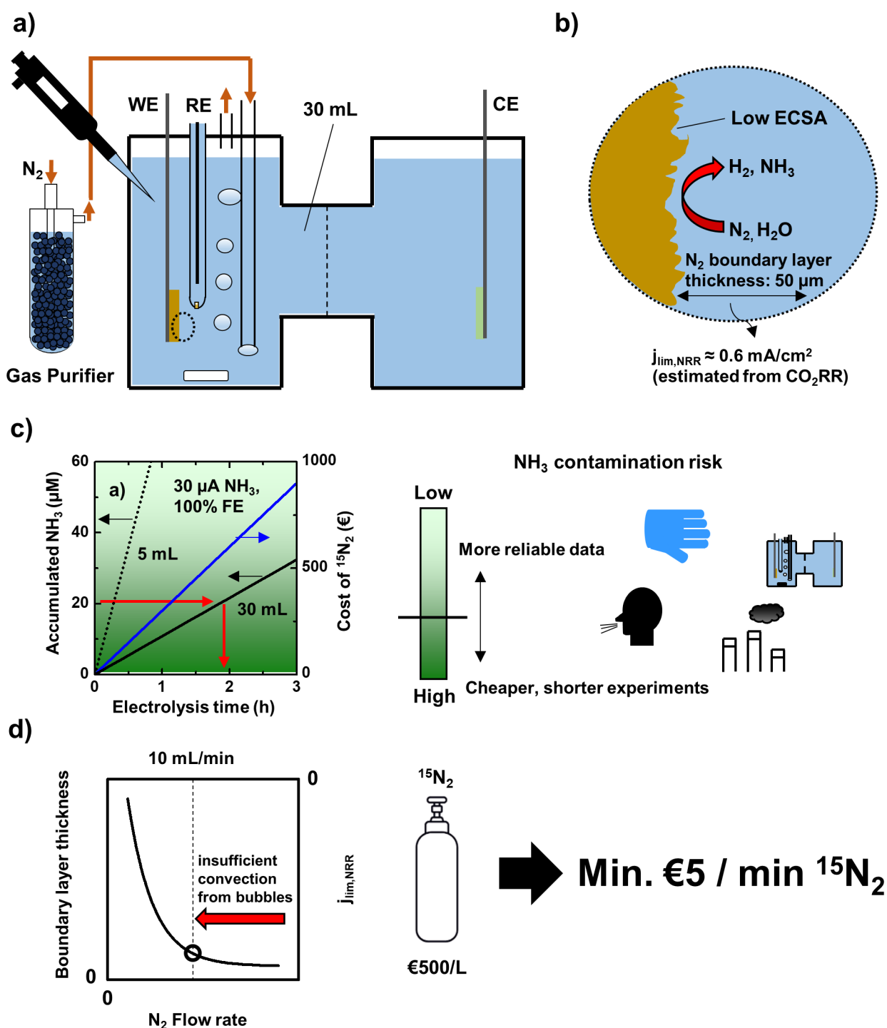
Figure 1. Limitations of H-cell cell design for NRR studies. (a) Schematic of an H-cell and gas purification. (b) Schematic of the electrode surface with 50 \mu\text{m} boundary layer and resulting mass-transport limiting current for NRR j_{\text{lim,NRR}} . (c) Dependence of the accumulated \text{NH}_3 and the cost of an isotope labeling experiment on the electrolysis time and the electrolyte volume. Ammonia production from NRR: 30 \mu\text{A} , flow rate during ^{15}\text{N}_2 experiments: 10 mL/min. The green color gradient represents the risk of \text{NH}_3 contamination (summarized from Table S2). (d) Dependence of \text{N}_2 mass transport to the cathode on the \text{N}_2 flow rate and resulting minimal cost of isotope labeling. Adapted from ref 26. Copyright 2018 American Chemical Society.
