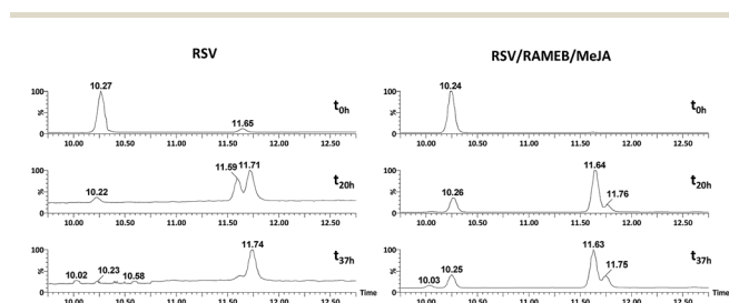
Fig. 12 UV traces at 286 and 306 nm of RSV (left) and RSV/RAMEB/MeJA (right) after UV exposure at t_0 h (top), t_{20} h (middle) and t_{37} h (bottom).
