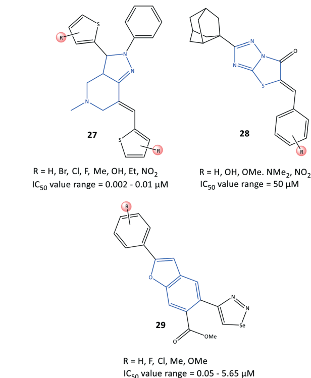
Fig. 25 Fused-ring derivatives 27, 28, and 29.
