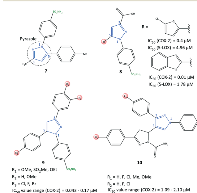
Fig. 12 Pyrazole-based inhibitors 7 , 8 , 9 , and 10 .
