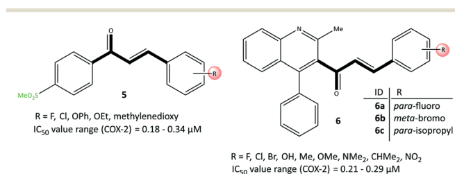
Fig. 11 Chalcone-based inhibitors 5 and 6 .
