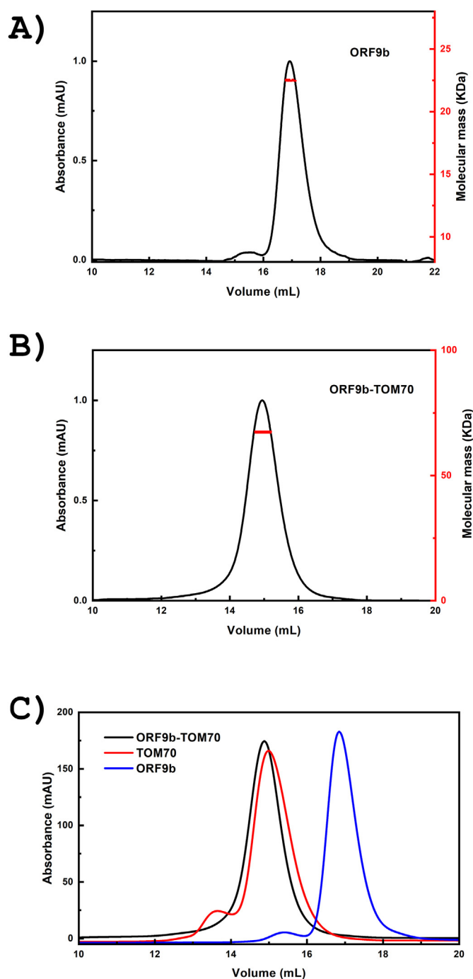
Fig. 2. Molecular mass determination A) ORF9b had a molecular mass of 22.0 \pm 1.0 kDa as indicated by SEC-MALS analysis. B) ORF9b-TOM70 had a molecular mass of 67.0 \pm 1.0 kDa, as indicated by SEC-MALS analysis. C) SEC-MALS profiles. Elution is dependent on the molecular mass, and ORF9b-TOM70 was eluted before TOM70 alone, indicating the formation of a complex.
