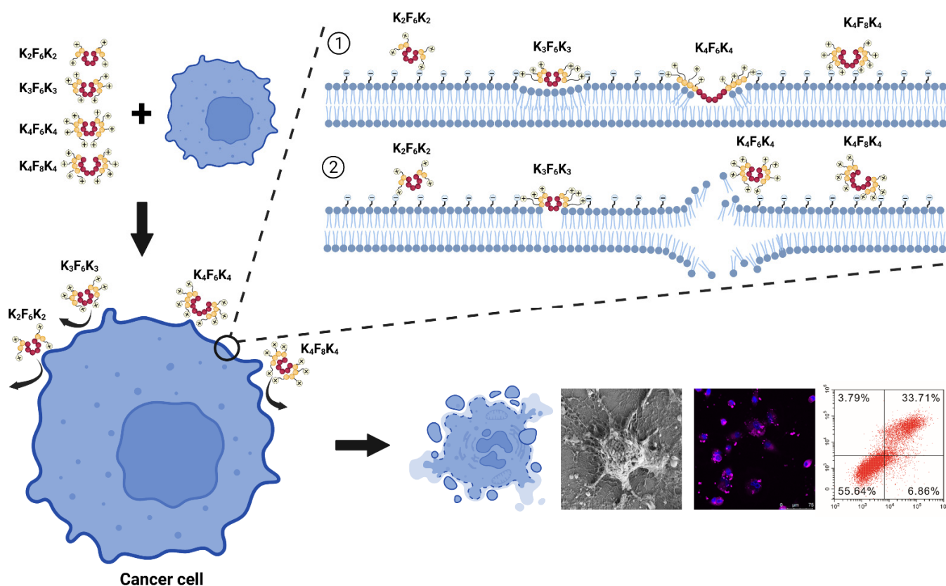
Figure 8. Schematic diagram of membrane disruption induced by K_nF_mK_n analogues ( K_2F_6K_2 , K_3F_6K_3 , K_4F_6K_4 , and K_4F_8K_4 ) against lung cancer cells A549. ① Firstly, the cationic K_nF_mK_n molecules were initially associated with the anionic cellular membranes via electrostatic interactions. During this process, increasing the cationic charging effects of K_nF_mK_n was found to promote antitumor activity. In addition, the tumor cells had elevated negative charges on the surface distinguished from noncancer cells; thus, K_4F_6K_4 could selectively kill A549 cells, but not HLF cells. ② Secondly, the hydrophobicity of phenylalanine residues in the middle promoted the interaction between the peptides and the fatty acyl chains to form pores, to align parallel to the surface on the cell membrane, and to disrupt the cell membrane. This may, in turn, result in irreversible cytolysis and finally the death of the target cells. The cell apoptosis assay by flow cytometry, the morphology observations using the optical microscope, the confocal microscopy with the CellMask™ Deep Red staining, and the scanning electron microscope identified this point. Of note, there was an optimal hydrophobicity needed for bioactivity; sequences with hydrophobicities below or very much above this threshold made the peptides inactive. Therefore, K_4F_8K_4 exhibited a much weaker cytotoxicity than that of K_4F_6K_4 under the same working conditions. Phenylalanine (F) is represented by the red spheres and lysine (K) is represented by the yellow spheres. The number of spheres indicates the number of corresponding amino acids.
