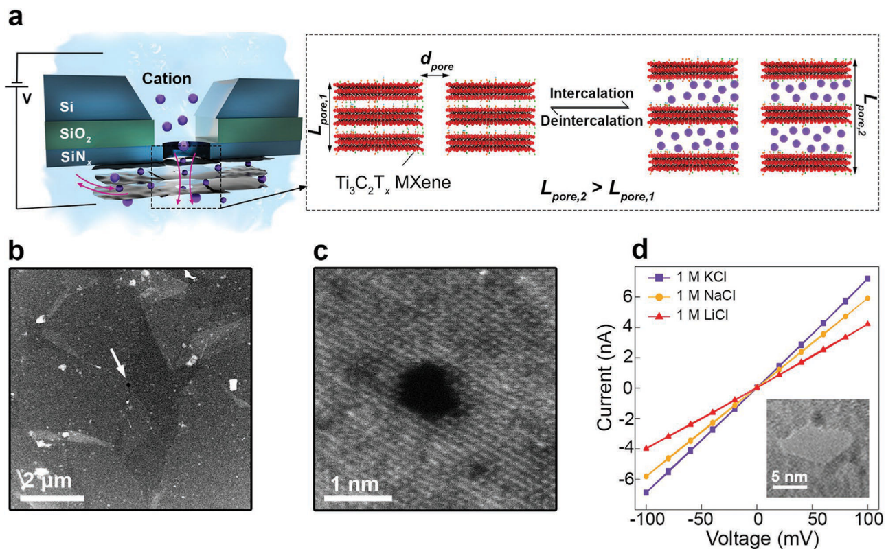
Figure 1. Ionic current detection through MXene nanopores. a) Schematic illustration of MXene nanopore experimental setup (left). A close-up look of the MXene nanopore and the effect of cation intercalation on the nanopore geometry (right). b) HAADF STEM image of a MXene film transferred on a SiN x membrane with a pre-fabricated aperture shown with an arrow. c) HAADF STEM image of a MXene nanopore fabricated with focused electron beam. d) Current–voltage curve of nanopore A in 1 m KCl (purple), 1 m NaCl (yellow), and 1 m LiCl (red). Inset shows the TEM image of the nanopore.
