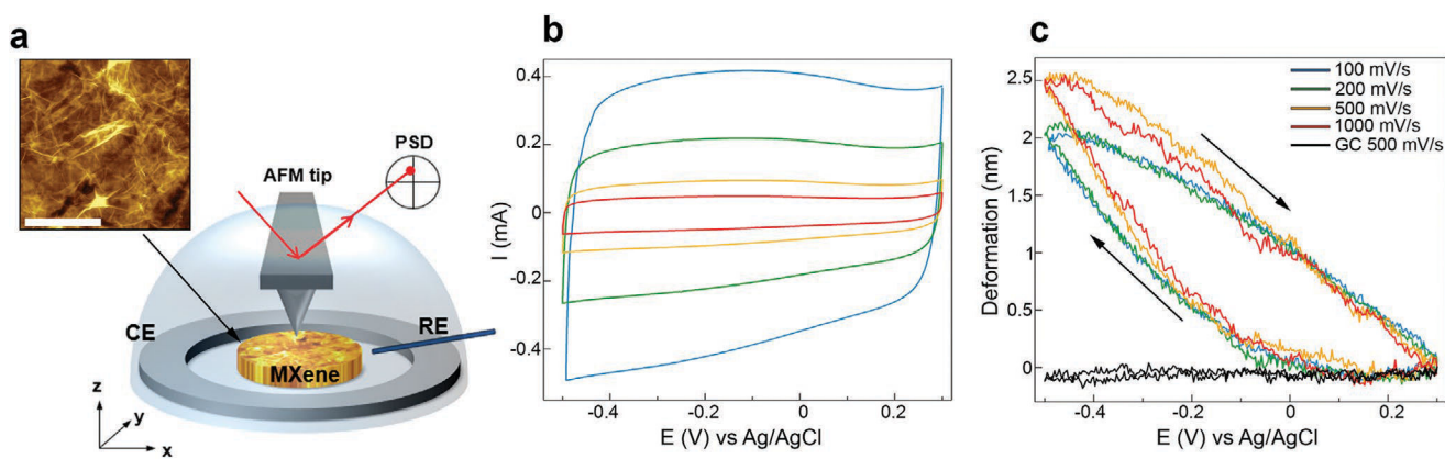
Figure 3. AFM dilatometry experiment of a deformation in a 16-layer MXene membrane. a) Illustration of operando AFM setup. AFM image scale = 4 μm. b) CV and c) deformation of a 16-layer MXene film in 0.5 m K 2 SO 4 at various scan rates.
