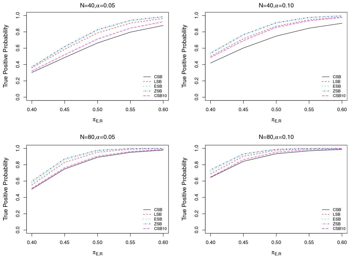
FIGURE 2. Plots of TPP for designs with constant stopping boundary (CSB, solid line), constant stopping boundary with first interim look at 10 patients (CSB10, longdashed line), linear stopping boundary (LSB, dashed line), exponential stopping boundary (ESB, dotted line), and zero stopping boundary (ZSB, dot-dashed line), respectively, as functions of true \pi_{E,R}^{\text{true}} changing from 0.40 to 0.60, for N=40 or 80 with m=5 , \pi_{S,R}^{\text{true}}=0.30 , \alpha=0.05 or 0.10
