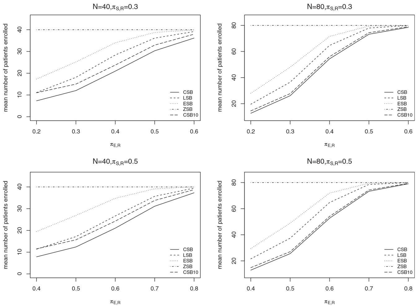
FIGURE 5. Plots of mean number of patients enrolled for designs with constant stopping boundary (CSB, solid line), constant stopping boundary with first interim at 10 (CSB10, longdashed line), linear stopping boundary (LSB, dashed line), exponential stopping boundary (ESB, dotted line), and zero stopping boundary (ZSB, dot-dashed line), respectively, as functions of true \pi_{E,R}^{\text{true}} changing from 0.20 to 0.60 or from 0.40 to 0.80, for N = 40 or 80 , \pi_{S,R} = 0.30 or 0.50 with m = 5 , \alpha = 0.05
