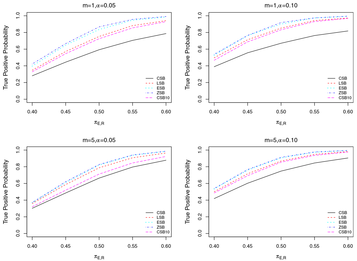
FIGURE 3. Plots of TPP for designs with constant stopping boundary (CSB, solid line), constant stopping boundary with first interim at 10 (CSB10, longdashed line), linear stopping boundary (LSB, dashed line), exponential stopping boundary (ESB, dotted line), and zero stopping boundary (ZSB, dot-dashed line), respectively, as functions of true \pi_{E,R}^{\text{true}} changing from 0.4 to 0.60, for m = 1 or 5 with N = 40 , \pi_{S,R}^{\text{true}} = 0.30 , \alpha = 0.05 or 0.10
