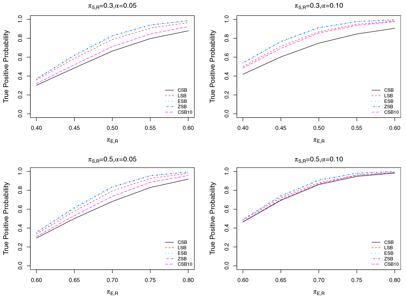
FIGURE 4. Plots of TPP for designs with constant stopping boundary (CSB, solid line), constant stopping boundary with first interim at 10 (CSB10, long dashed line), linear stopping boundary (LSB, dashed line), exponential stopping boundary (ESB, dotted line), and zero stopping boundary (ZSB, dot-dashed line), respectively, as functions of \pi_{E,R}^{\text{true}} changing from 0.40 to 0.60 or from 0.60 to 0.80, for \pi_{S,R}^{\text{true}} = 0.30 or 0.50 with N = 40 , m = 5 , \alpha = 0.05 or 0.10
