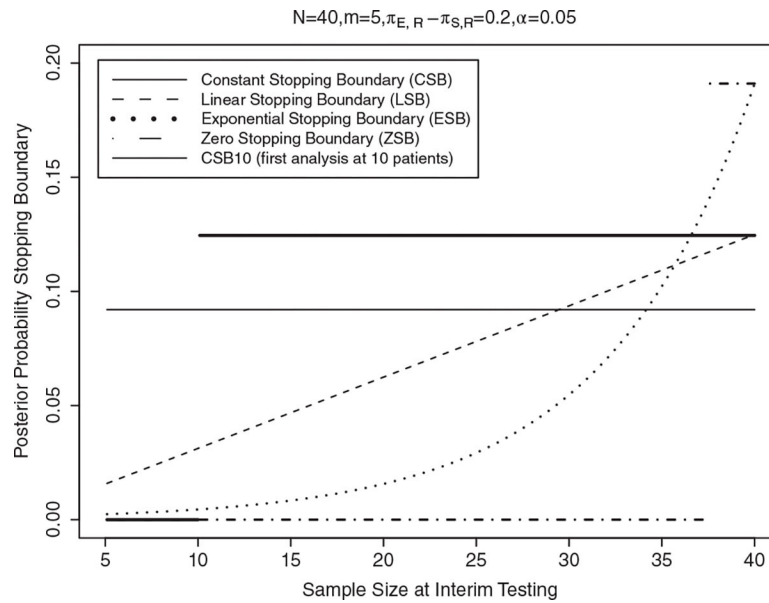
FIGURE 1. Futility stopping boundaries at each interim analysis ( n = 5, 10, \dots, 40 ) for the five designs: Constant stopping boundary (CSB, thin solid line), Constant stopping boundary with first interim at 10 (CSB10, thick solid line), linear stopping boundary (LSB, dashed line), exponential stopping boundary (ESB, dotted line), and no early stopping (or Zero Stopping Boundary, ZSB, dot-dashed line), respectively, under N = 40, m = 5, \pi_{S,R} = 0.30, \delta = 0.2, \alpha = 0.05
