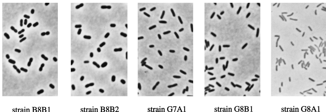
FIG. 1. Phase-contrast photomicrographs of new denitrifying isolates grown with dimethylmalonate (5 mM) and nitrate (10 mM). Bar, 10 \mu\text{m} .
