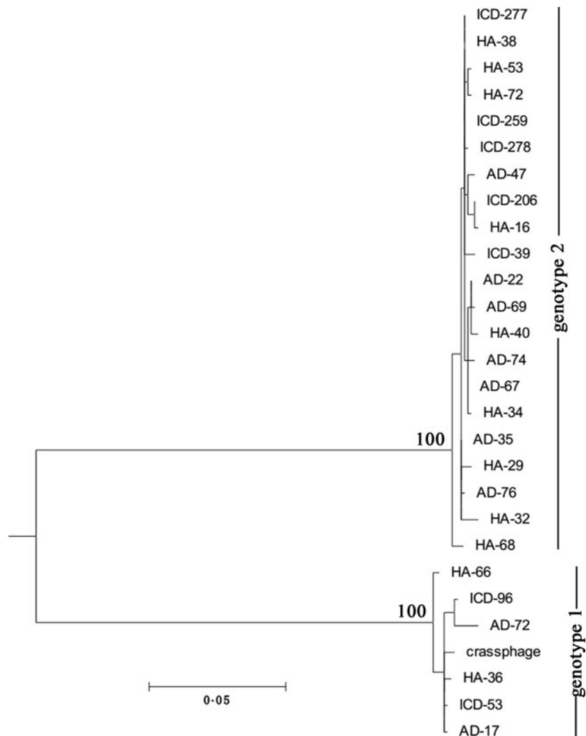
Fig. 1. Phylogenetic analysis by maximum likelihood based on the partial-length ORF00018 gene (846 bp). Bootstrap values in the bootstrap test with 1000 replications were shown on the key nodes of the tree. The scale bar (0.05) indicated substitutions per site. ICD, Infants/children with diarrhoea; AD, adults with diarrhoea; HA, healthy adults. The GenBank accession number of crAssphage is NC_024711.
