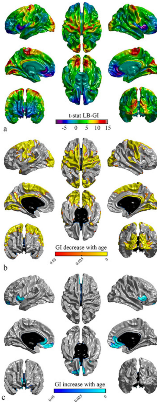
Fig. 6. Statistical maps of gyrification values for LB-GI, projected on different views of the brain. Left panel: left lateral view (top), medial view of left hemisphere (middle), anterior view (bottom). Middle panel: superior view (top), inferior view (bottom). Right panel: right lateral view (top), medial view of right hemisphere (middle), posterior view (bottom). a) T -statistic maps for an age effect on decrease in gyrification. b) Illustration of the regions of significantly decreased gyrification with age (warm colors). c) The regions of significantly increased gyrification with age (cool colors). Vertex level p -values ( p <
