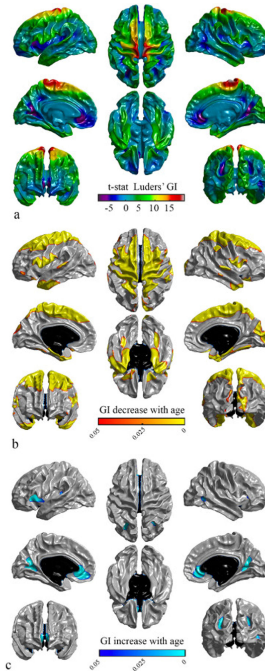
Fig. 7. Statistical maps of gyrification values for Luders' GI, projected on different views of the brain. Left panel: left lateral view (top), medial view of left hemisphere (middle), anterior view (bottom). Middle panel: superior view (top), inferior view (bottom). Right panel: right lateral view (top), medial view of right hemisphere (middle), posterior view (bottom). a) T -statistic maps for an age effect on decrease in gyrification. b) Illustration of the regions of significantly decreased gyrification with age (warm colors). c) The regions of significantly increased gyrification with age (cool colors). Vertex level p -values ( p < 0.05 ) are corrected
