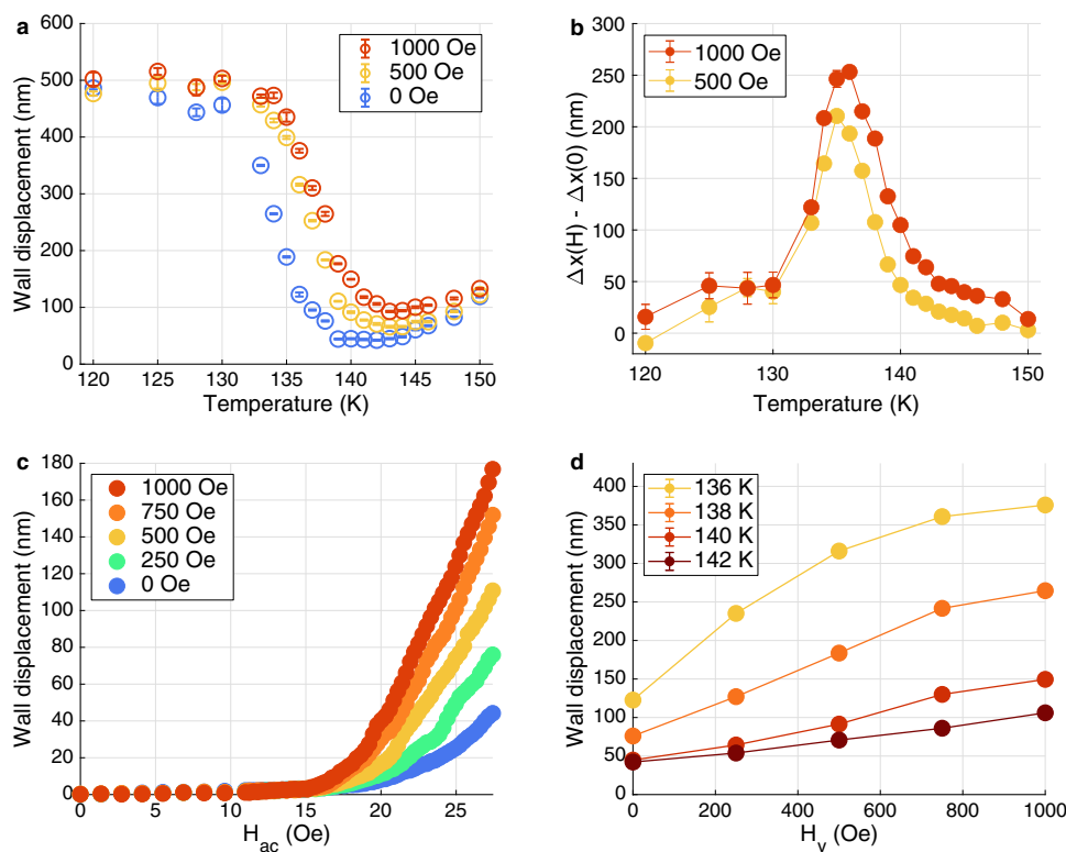
Fig. 3 Magnetic field dependence of the DW ellipticity. a DW displacement plotted against temperature for various in-plane dc magnetic field H_y , applied to the sample. b The changes in DW displacement \Delta x induced by dc field values of H_y = 500 Oe and 1000 Oe show sharp peaks at T = 135 K and 136 K, indicating a phase transition into the linear wall state, c DW displacement versus H_{ac} for different values of in-plane dc fields H_y at T = 139 K. A clear change in the DW displacement and mobility is observed by tuning the wall ellipticity with an in-planned field H_y , applied to the sample near T_{BG} . d DW displacement plotted versus in-plane field H_y for various temperatures. A saturation behavior is observed at lower temperatures toward the Bloch wall phase.
