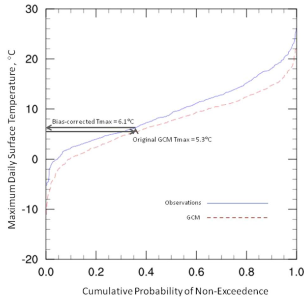
Fig. 3 Example CDF for maximum daily near-surface temperature. Arrows illustrate the quantile mapping process used for bias correction. Adapted from Thrasher, et al. , 2012.
