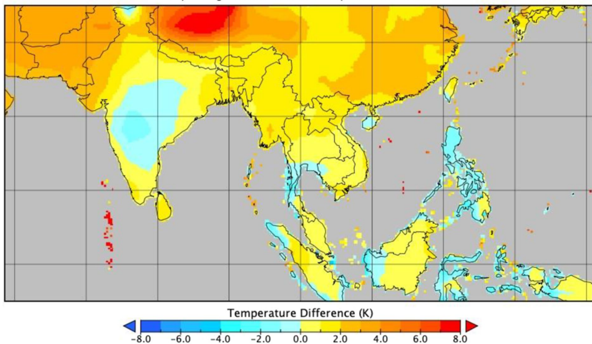
Fig. 1 End of century daily average maximum near-surface air temperature difference between the downscaled CanESM5 model output (CMIP6) and the corresponding downscaled CanESM2 model output (CMIP5).
