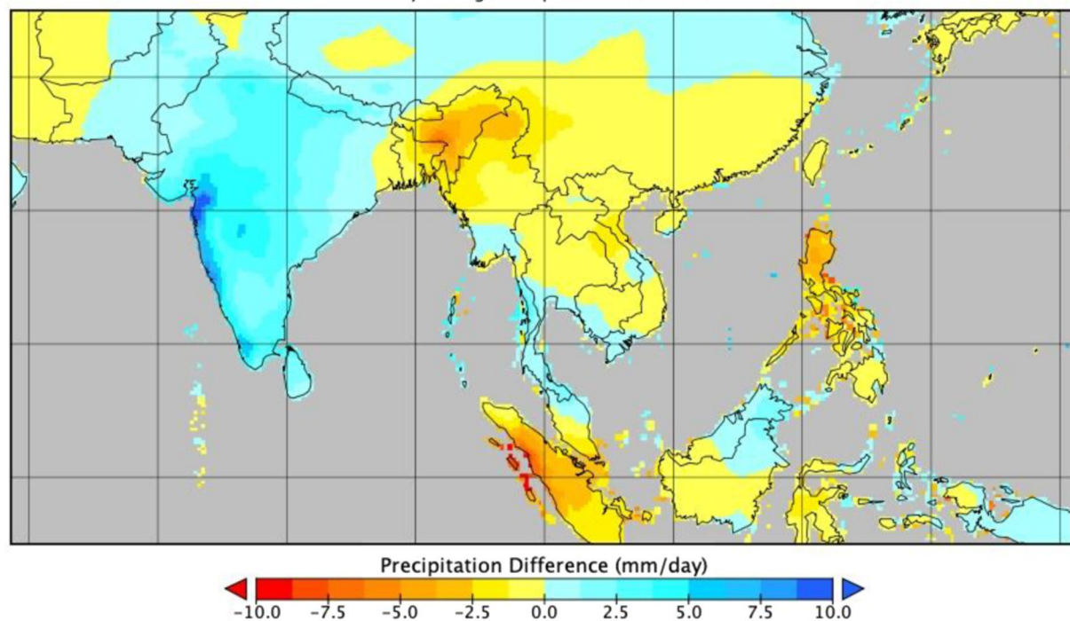
Fig. 2 Same as Fig. 1, but for precipitation.
