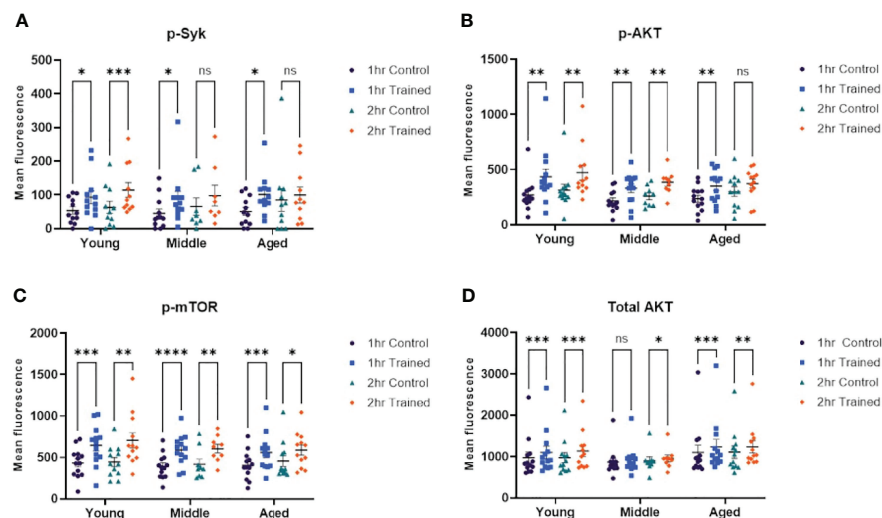
FIGURE 5 | Immune training activates intracellular signaling pathways in monocytes. (A) Scatterplot depicting phosphorylated-Syk 1 and 2 hours after \beta -glucan or PBS treatment (N=8–12). (B) Scatterplot depicting phosphorylated-AKT expression (N=9–13). (C) Scatterplot depicting phosphorylated-mTOR (N=9–13). (D) Scatterplot depicting total AKT expression (N=9–13). All results analyzed using a mixed-effect model and Šidák's multiple comparisons test (* P \leq 0.05 , ** P \leq 0.01 , *** P \leq 0.001 , **** P \leq 0.0001 , ns, not significant).
