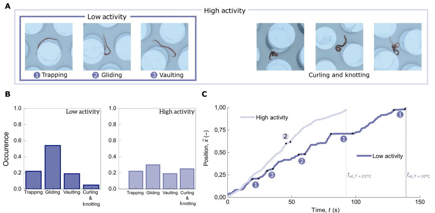
Fig. 4. Effect of active-worm conformations on the transport through a pillar array. (A) Photographs showing the typical conformations at a high level of activity ( T=25^\circ C , light blue) and restricted to fewer conformations at low activity (i.e., low temperature or in the presence of alcohol, dark blue). (B) Conformation statistics. The worm conformations have been measured along the elution in the channel for two different levels of activity. (C) Tracked position of the active worm along the length of the channel \bar{x} = \frac{x}{(x_f - x_0)} for two different levels of activity as a function of time. Conformations of the active worms influence the elution time in the channel. At low level of activity, modes (1 to 3) are dominant, which increases the elution time.
