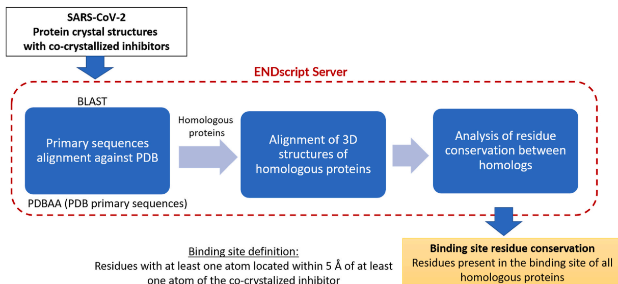
Fig. 1. General workflow of the protein binding sites comparison. The ENDscript server ( https://endscript.ibcp.fr/ESPrift/ENDScript/ ) was employed; it is publicly accessible tool for multiple sequence alignment of proteins homologous to the query, alignment of their corresponding crystal structures, and coloring the query structure according to residue conservation (Robert and Gouet, 2014).
