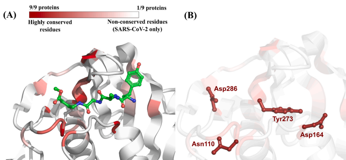
Fig. 2. (A) Color-coded depiction of residue conservation at the binding site of all identified SARS-CoV-2 PL PRO homologous proteins. Regions in dark red represent residues with high co-occurrence among homologous proteins (i.e., nine out of nine proteins share the same residue). Regions in light red represent residues with moderate co-occurrence (i.e., between 2 and 8 out of nine proteins share the same residue). Regions in white represent residues with no co-occurrence (i.e., the residue is present only in SARS-CoV-2). The protein structure used as template is the PL PRO from SARS-CoV-2 (PDB ID: 6WX4) co-crystallized with the peptide-like inhibitor VIR251 (in green) (Rut et al., 2020); (B) Binding site residues of SARS-CoV-2 PL PRO conserved in all homologous proteins listed in Table 1.
