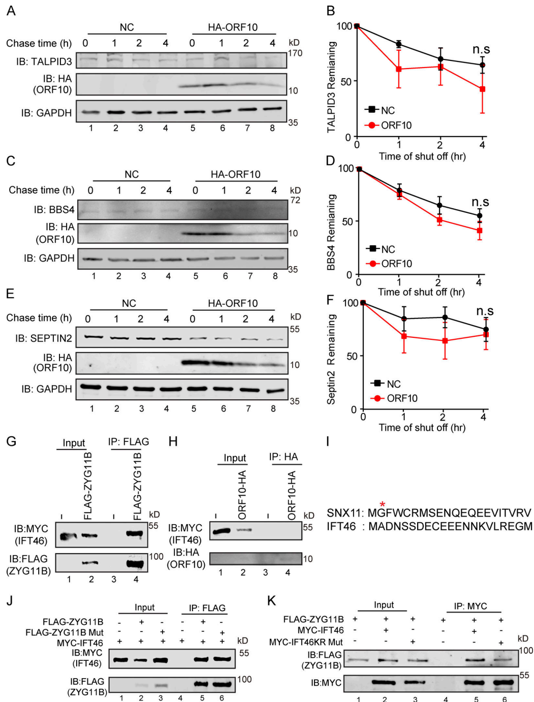
Figure S4. The interaction of ZYG11B and IFT46 is not based on a Gly/N-degron-based mechanism. (A, C, and E) A cycloheximide chase (CHX) assay of TALPID3, BBS4, and SEPTIN2 was performed in ORF10-expressing and empty vector control HEK293T cells. Samples were taken at 0, 1, 2, and 4 h after the addition of CHX. The TALPID3, BBS4, SEPTIN2, and ORF10 protein levels were detected by immunoblotting using TALPID3, BBS4, SEPTIN2 antibodies, and HA antibody. GAPDH served as a loading control. (B, D, and F) Quantification of the TALPID3, BBS4, and SEPTIN2 levels in (A, C, and E). The protein level of TALPID3, BBS4 and SEPTIN2 was quantified using Odyssey software. (n = 3 independent experiments). Data are presented as the mean ± SEM. Statistical analysis was performed with two-tailed unpaired Student's t test. (G) ZYG11B physically interacts with IFT46. MYC-IFT46 and ZYG11B-FLAG (or empty vector) were co-transfected into HEK293T cells. 24 h after transfection, cells were collected for immunoprecipitation (IP) with an anti-FLAG antibody, followed by analysis using anti-FLAG and anti-MYC antibodies. (H) ORF10 could not interact with IFT46. MYC-IFT46 and ORF10-HA (or empty vector) were co-transfected into HEK293T cells. 24 h after transfection, cells were collected for immunoprecipitation (IP) with an anti-HA antibody, followed by analysis using anti-HA and anti-MYC antibodies. (I) The protein sequences of SNX11 and IFT46. (J) ZYG11B-Mut did not affect the interaction of IFT46 and ZYG11B. MYC-IFT46 and ZYG11B-FLAG (or ZYG11B-Mut-FLAG) were co-transfected into HEK293T cells. 24 h after transfection, cells were collected for immunoprecipitation (IP) with an anti-FLAG antibody, followed by analysis using anti-FLAG and anti-MYC antibodies. (K) IFT46 KR Mut did not affect the interaction of IFT46 and ZYG11B. ZYG11B-FLAG and MYC-IFT46 (or IFT46 KR Mut) were co-transfected into HEK293T cells. 24 h after transfection, cells were collected for immunoprecipitation (IP) with an anti-MYC antibody, followed by analysis using anti-FLAG and anti-MYC antibodies. Source data are available for this figure: SourceData FS4.
