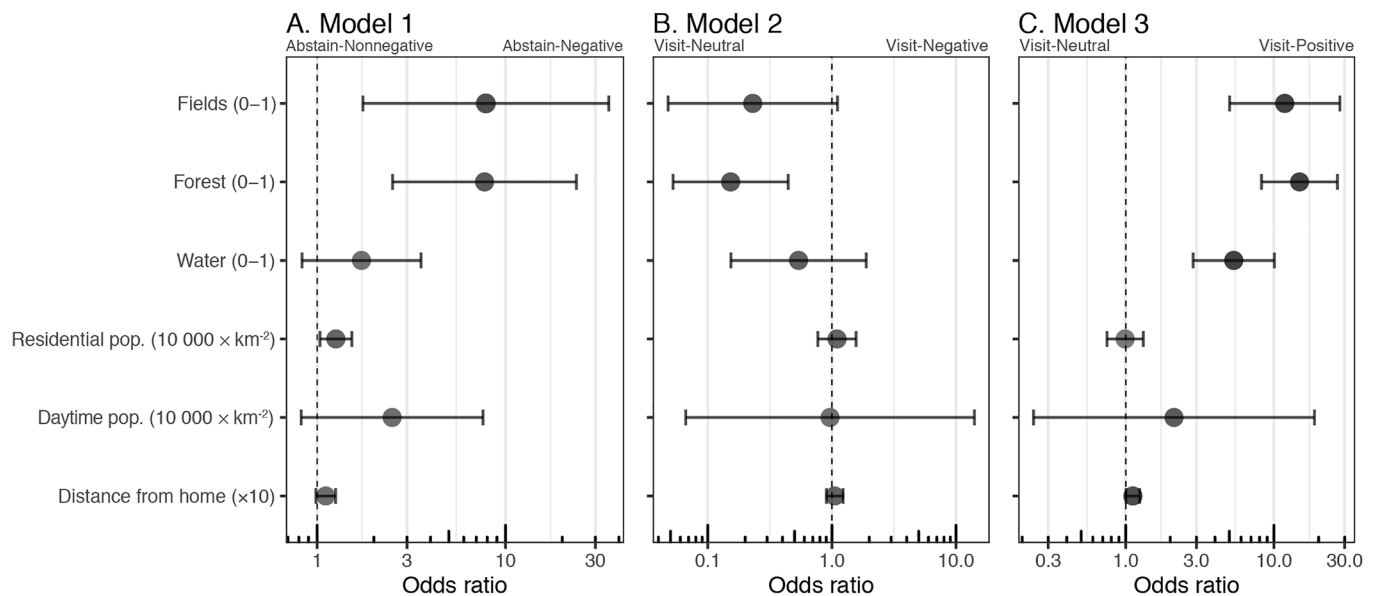
Fig. 5. Associations between geographical and sociodemographic properties of places and wellbeing outcomes of their use, as estimated in spatial logistic regression Model 1: Abstain-Negative versus Abstain-Nonnegative (A), Model 2: Visit-Negative versus Visit-Neutral (B) and Model 3: Visit-Positive versus Visit-Neutral (C). Associations are shown as odds ratios (dots) with 95% confidence intervals (bracketed lines). Units used in the models are given within brackets. (A) Abstaining from visiting places is more likely to have a negative influence on wellbeing when they have natural features and are in areas with many residents. (B) Visiting places similarly or more often is more likely to have a negative influence on wellbeing if they do not contain forest. (C) Visiting places similarly or more often is more likely to have a positive influence on wellbeing when they feature fields, forests and water.
