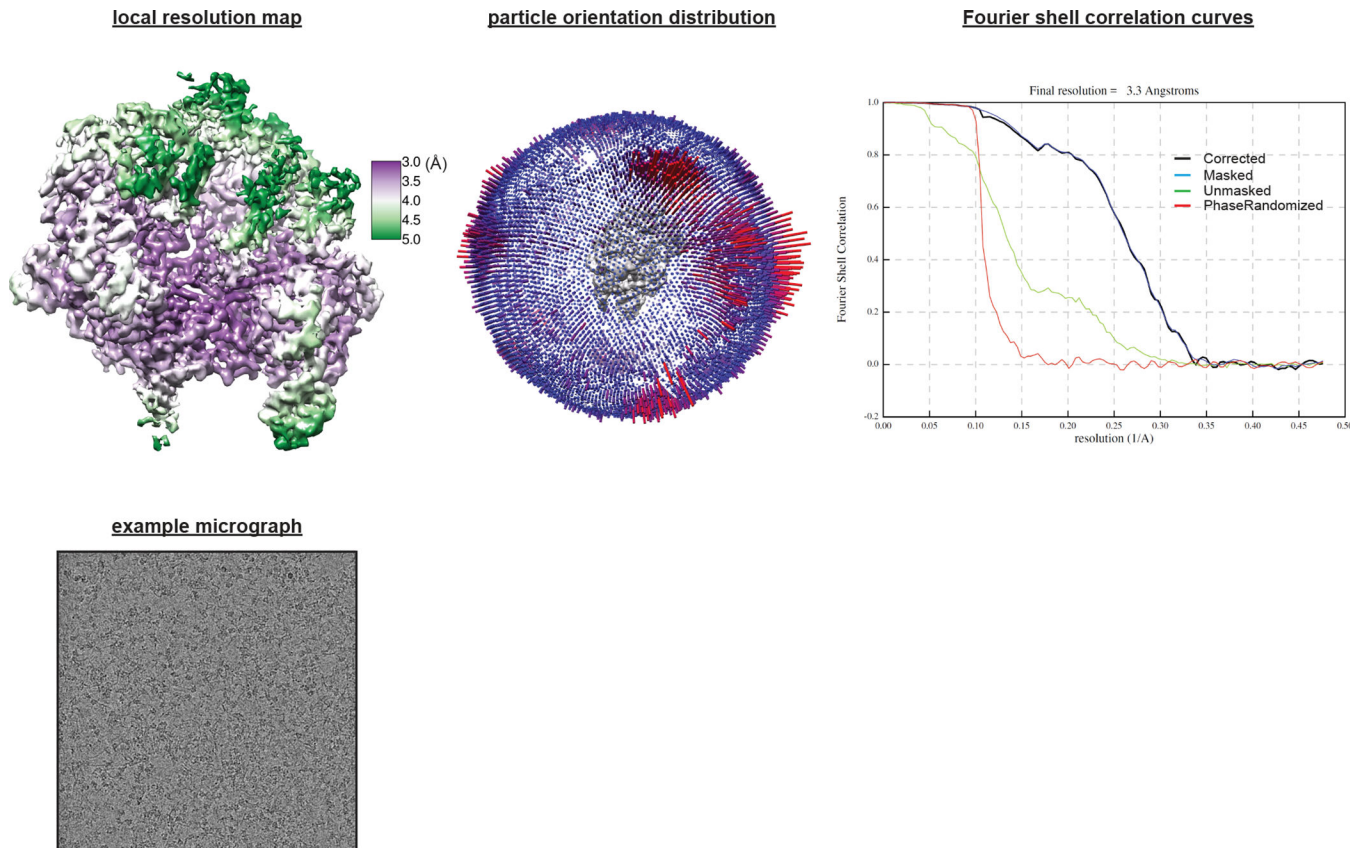
Extended Data Fig. 9. Cryo-EM analysis of Cas9:sgRNA:DNA with 3 RNA:DNA matches. Details of cryo-EM analysis.
