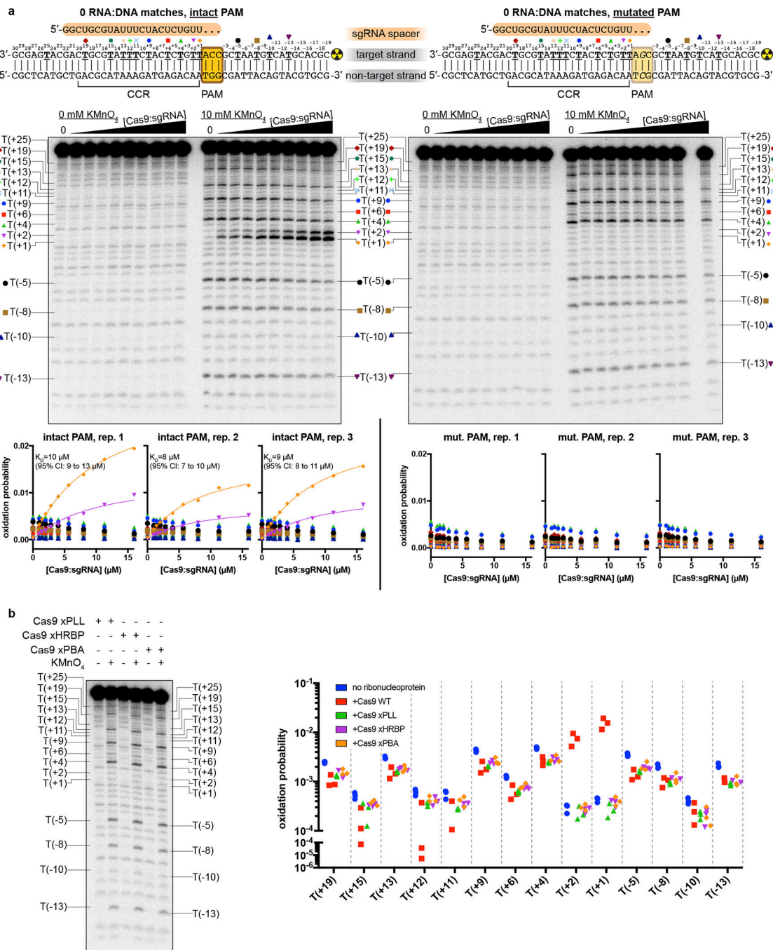
Extended Data Fig. 7. Details of permanganate reactivity measurements.
