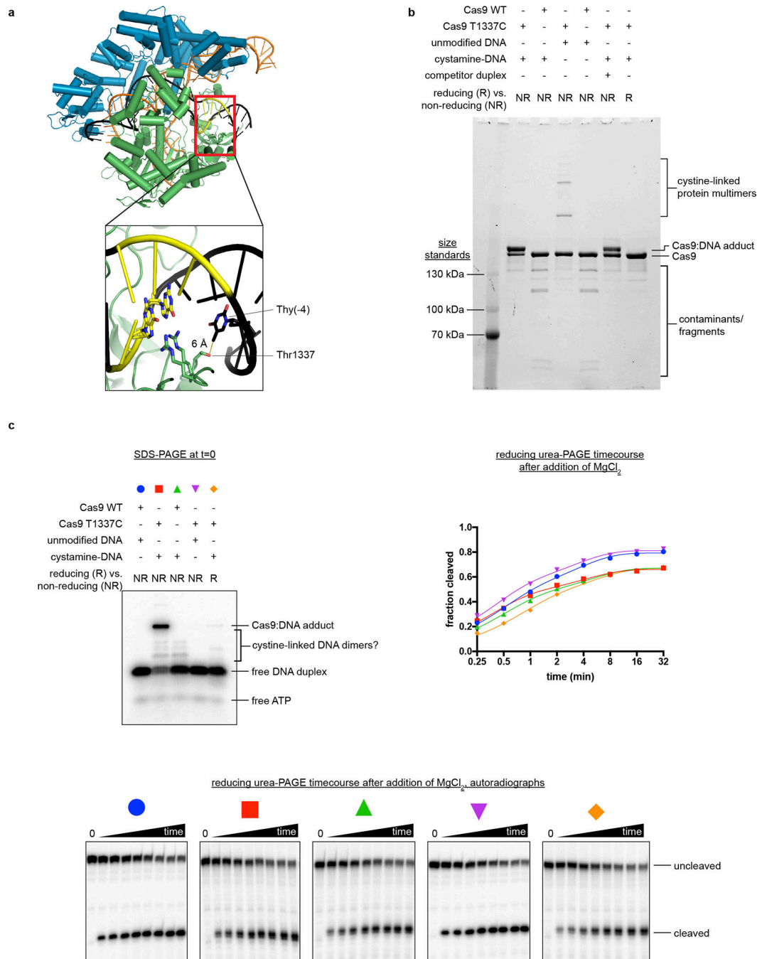
Extended Data Fig. 1. Characterization of the Cas9:DNA cross-link.
