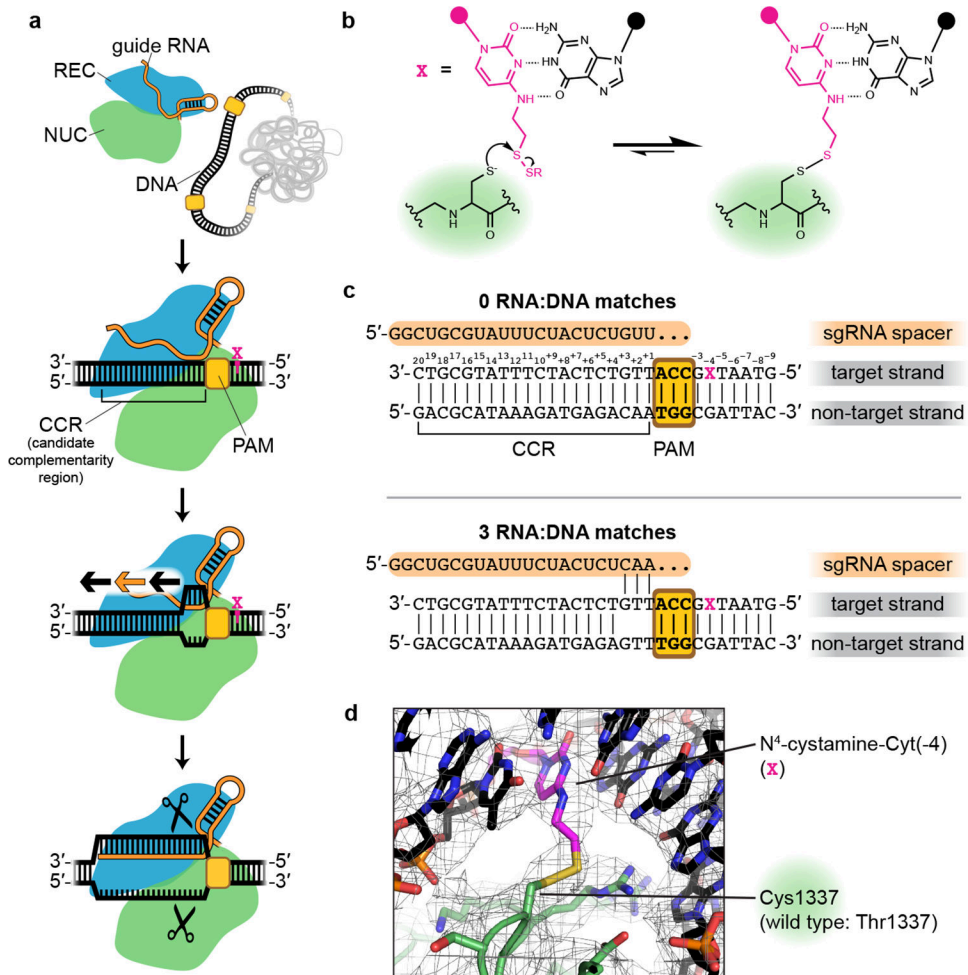
Fig. 1 |. Trapping the Cas9 interrogation complex.
