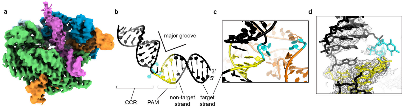
Fig. 3 |. DNA conformation at the site of bending.
