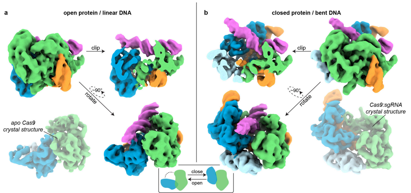
Fig. 2 | Cryo-EM structures of the Cas9 interrogation complex, compared to previously determined crystal structures.
