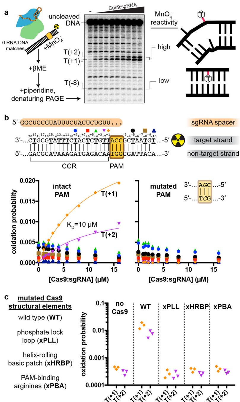
Fig. 5 |. Permanganate reactivity measurements.
