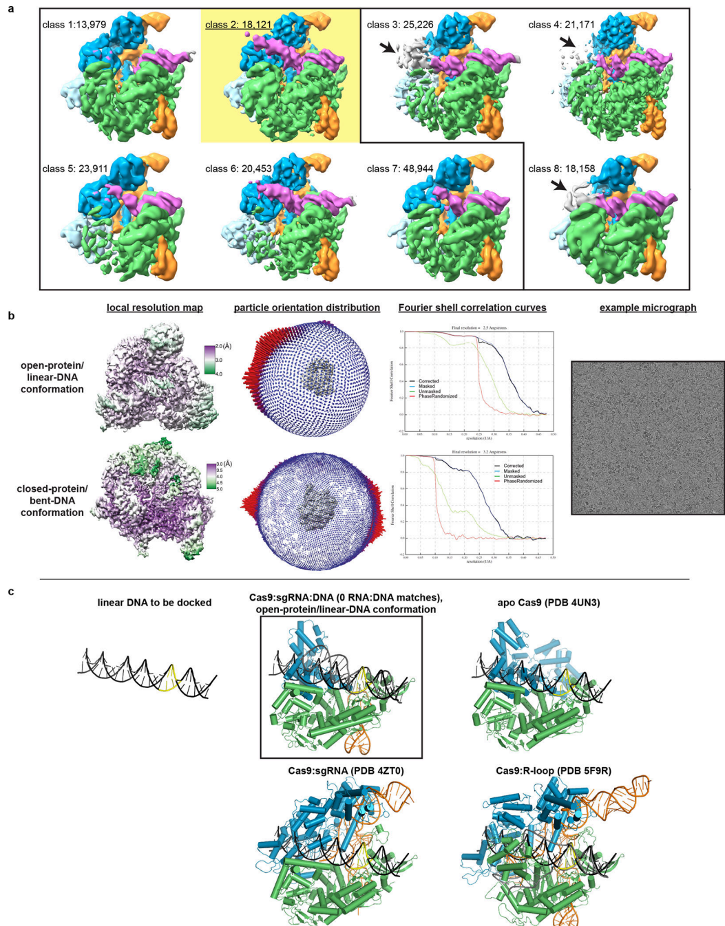
Extended Data Fig. 3. Cryo-EM analysis of Cas9:sgRNA:DNA with 0 RNA:DNA matches. a , Classes from RELION 3D classification of closed-protein particles (threshold 6\sigma ). The number of particles in each class is indicated next to the class number. In classes 1/2/5/6/7
