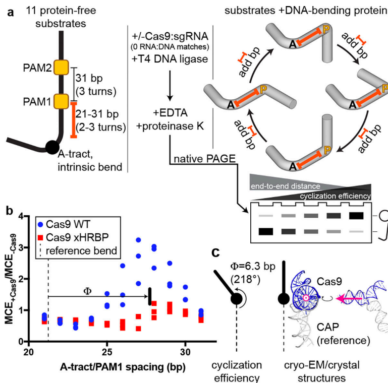
Fig. 4 | DNA cyclization efficiency experiments.
