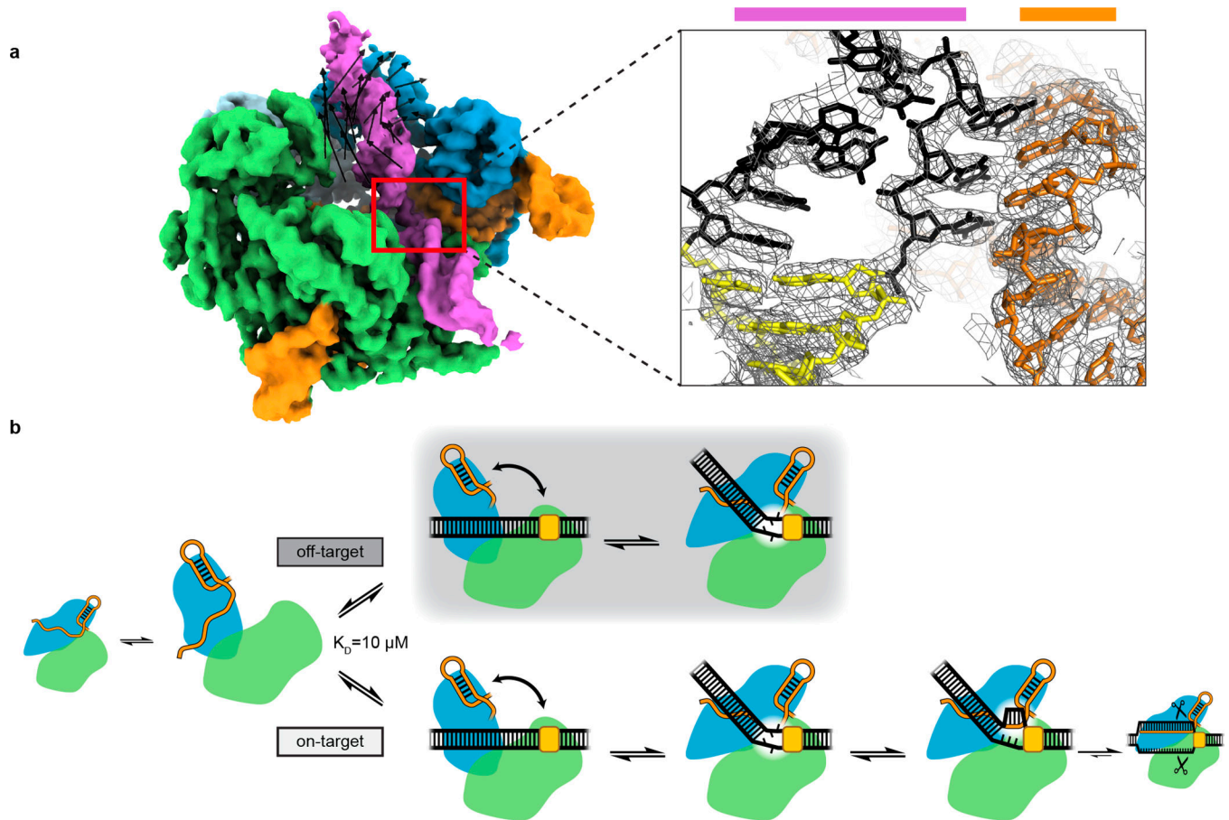
Fig. 6 |. Structure of a nascent R-loop and overview model.
