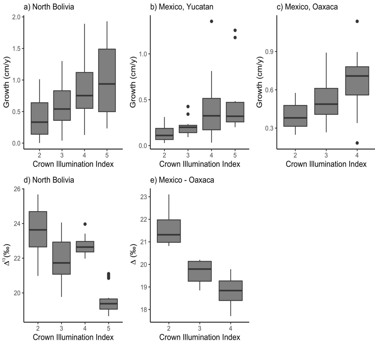
Figure 3. Diameter growth rate and isotope discrimination ( \Delta^{13}C_{tr} ) in relation to crown illumination index (CII). The CII varies from 2 for sapling and seedlings without direct sunlight to 4 and 5 for trees with full direct sunlight from above or for emergent crowns. Both growth and isotope discrimination are calculated as the mean over the past five rings for extant trees. Boxes denote 25th, 50th and 75th percentile and whiskers extend to the largest or smallest value no more than 1.5 times the interquartile range. Letters indicate significant ( P < 0.05 ) differences between CII classes using paired t -tests. In all three sites, CII explains greater amount of variation than diameter using ANOVA with tree diameter as covariable.
