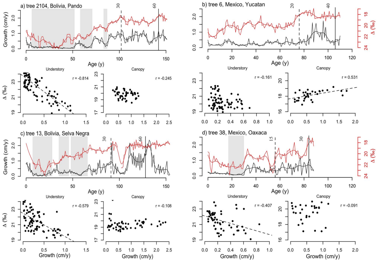
Figure 4. Examples of trajectories for growth (black lines) and C-isotope discrimination ( \Delta^{13}C , red lines in reversed axes) of individual trees, and scatterplots of growth versus \Delta^{13}C for understory and canopy growth phases. Note the reverse axis for \Delta^{13}C time series in red in the upper panels. Understory is defined as trees smaller than 30, 20 and 15 cm in diameter for Bolivia, Yucatan and Oaxaca, respectively, which is the approximate size at which trees reach the lower canopy (see Materials and methods). The age at which the individual trees reached these diameter thresholds for understory versus canopy growth phases or larger canopy sizes are indicated in the trajectory plots with vertical broken and continuous lines, respectively, with numbers referring to tree diameter in cm. The trend lines in the scatter plots indicate significant ( P < 0.05 ) relationships between early growth rate and \Delta^{13}C , and Pearson correlation coefficients ( r ) are shown. Smooth curves for growth and \Delta^{13}C trajectories are smoothing splines (see Materials and methods). Periods of suppression (i.e., minimum of 5 years of growth below a site-specific threshold, see Materials and methods) are indicated by shaded areas.
