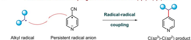
Fig. 2 Strategy for a metal-free deoxygenative C(sp^3)-C(sp^2) coupling of alcohols and pyridines.
