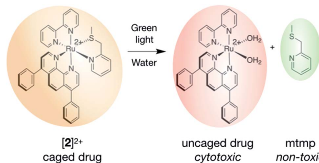
Fig. 1 Activation mechanism of the ruthenium-based PACT compound [2]^{2+} . Upon green light irradiation, the protecting, non-toxic mtmp ligand is photosubstituted by solvent molecules, which recovers the biomolecule-binding ability of the heavy metal centre, ultimately leading to cytotoxicity and cell death.
